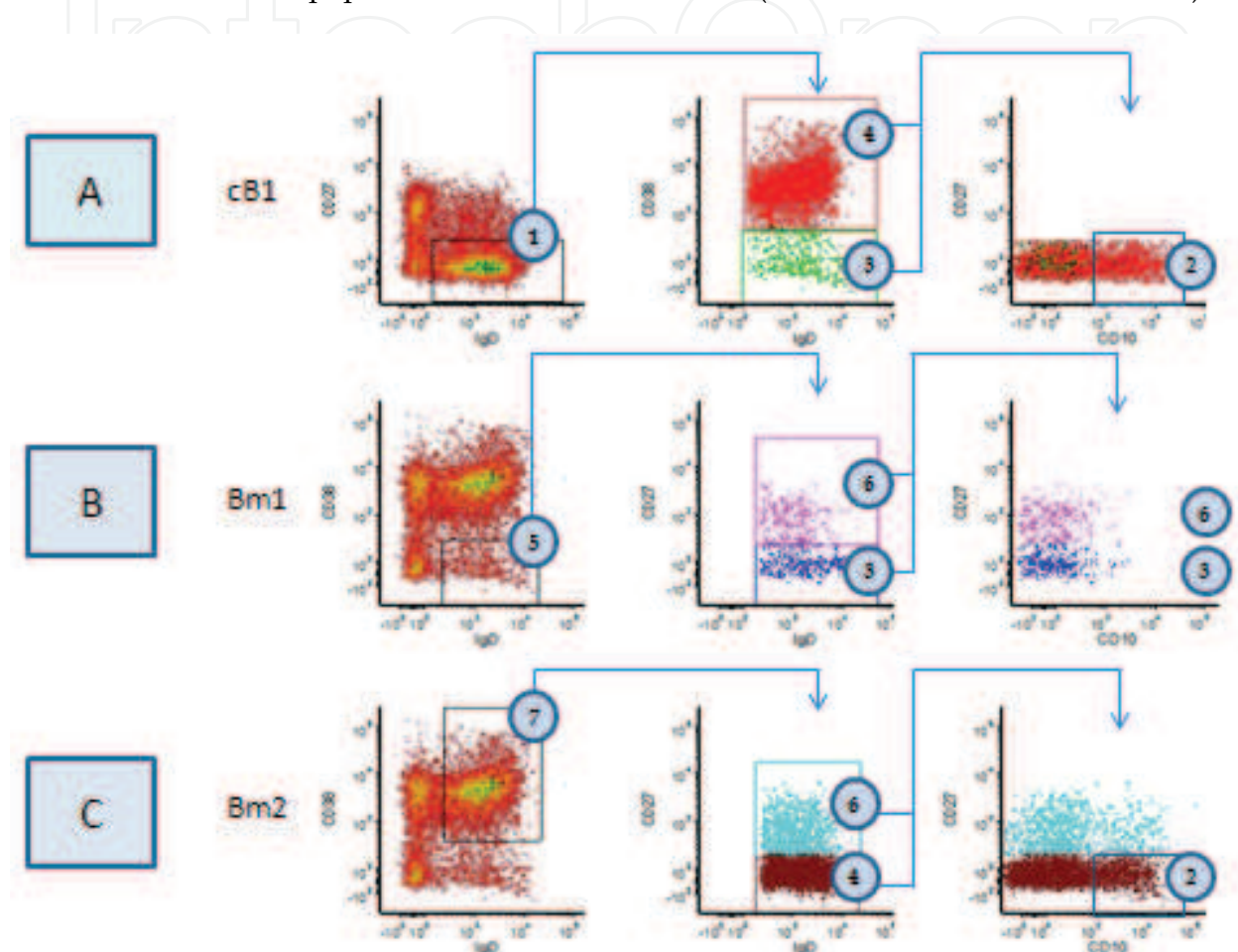
Fig. 4. Limitations of using cB1 and Bm1/2 in isolation to define the naïve B cell population. Blood from one healthy subject with recent influenza vaccination is shown. B cells are initially gated using CD45+ and co-expression of CD19+ and CD20+. IgD, CD27, CD38 are used to capture naïve B cells using both classification systems. Subpopulations are backgated to visualize heterogeneity in reciprocal classification schemes. Additionally, each classification scheme (cB1, Bm1, Bm2) is shown using CD10 and CD27 to identify CD10+CD27- transitional B cells. A) cB1 ① (IgD+CD27-) consists of transitional cells (CD10+CD27-) ② as well as mature naïve (IgD+CD27-CD38-CD10-) B cells ③ and activated naïve (IgD+CD27-CD38+CD10-) B cells ④. B) Bm1 ⑤ (IgD+CD38-) consists of mature naïve (IgD+CD27-CD38-CD10-) B cells ③ and non-class switched memory (IgD+CD27+CD10-) B cells ⑥. C) Bm2 ⑦ (IgD+CD38+) consists of transitional cells (CD10+CD27-) ② as well as activated naïve (IgD+CD27-CD38+CD10-) B cells ④ and non-class switched memory (IgD+CD27+CD10-) B cells ⑥
