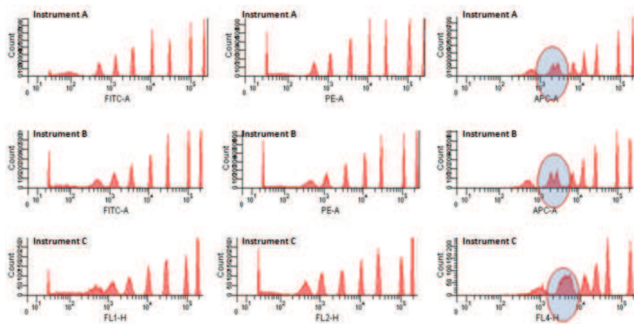
Fig. 6. Sensitivity varies between instruments. SPHERO™ Ultra Rainbow beads were acquired using optimal instrument settings on 3 different flow cytometers. Resolution of the dim peaks in the APC channel on Instrument C is inferior to Instrument A and B
