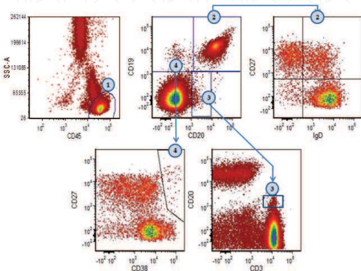
Fig. 2. Establishing the B cell gate. Blood from one healthy donor with recent influenza vaccination is shown to demonstrate B cell lineage gate. CD45 is used to discriminate leukocytes (1) from red blood cells and debris. Co-staining with CD19 and CD20 separates B cells (2) from dim CD20 expressing T cells (3) and CD20 negative plasmablasts/cells (4)
