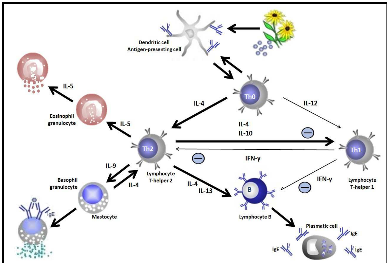
Fig. 1. Mechanism of allergic reaction.
