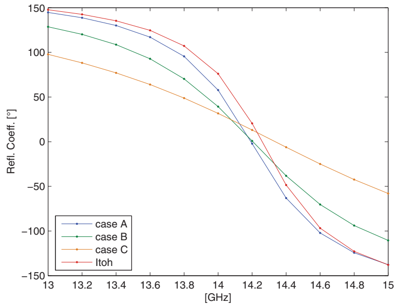
Fig. 13. Reflection Coefficient.
