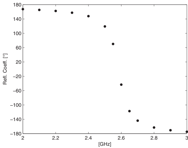
(b) Reflection Coefficient
