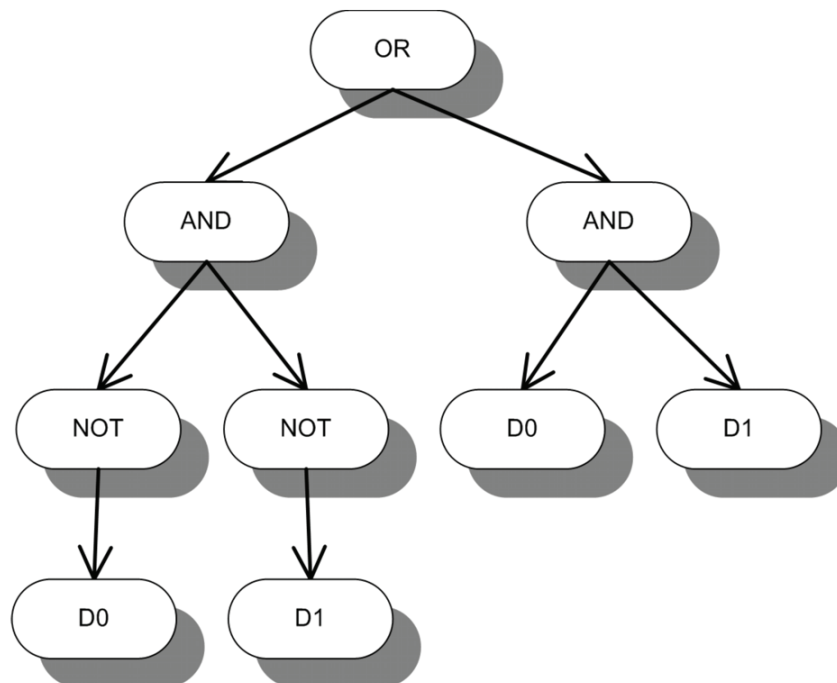
Fig. 2. S-expression: tree architecture.
