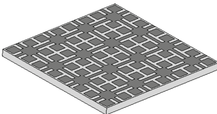
Fig. 1. Uniplanar Compact Photonic Band-Gap (UC-PBG)(Yang et al., 1999)
