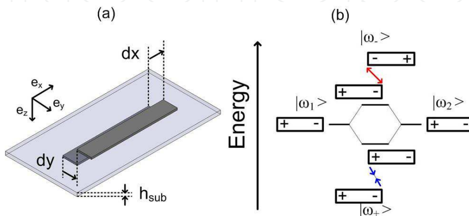
Fig. 2. (a) Asymmetric cut-wire pair with the three degrees of freedom for the control of the coupling strength: h_{sub} , dx and dy . (b) Inverted hybridization scheme.
