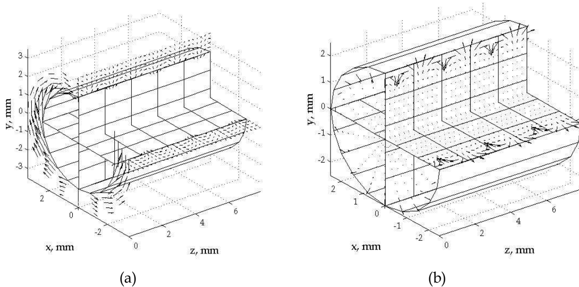
Fig. 3.3. The 3D electric field distributions of the main of circular metamaterial waveguide with r=2.5 mm at f=110 GHz. (a) - the electric field strength lines outside the waveguide (b) - the 14 times were increased electric field strength lines inside the waveguide
