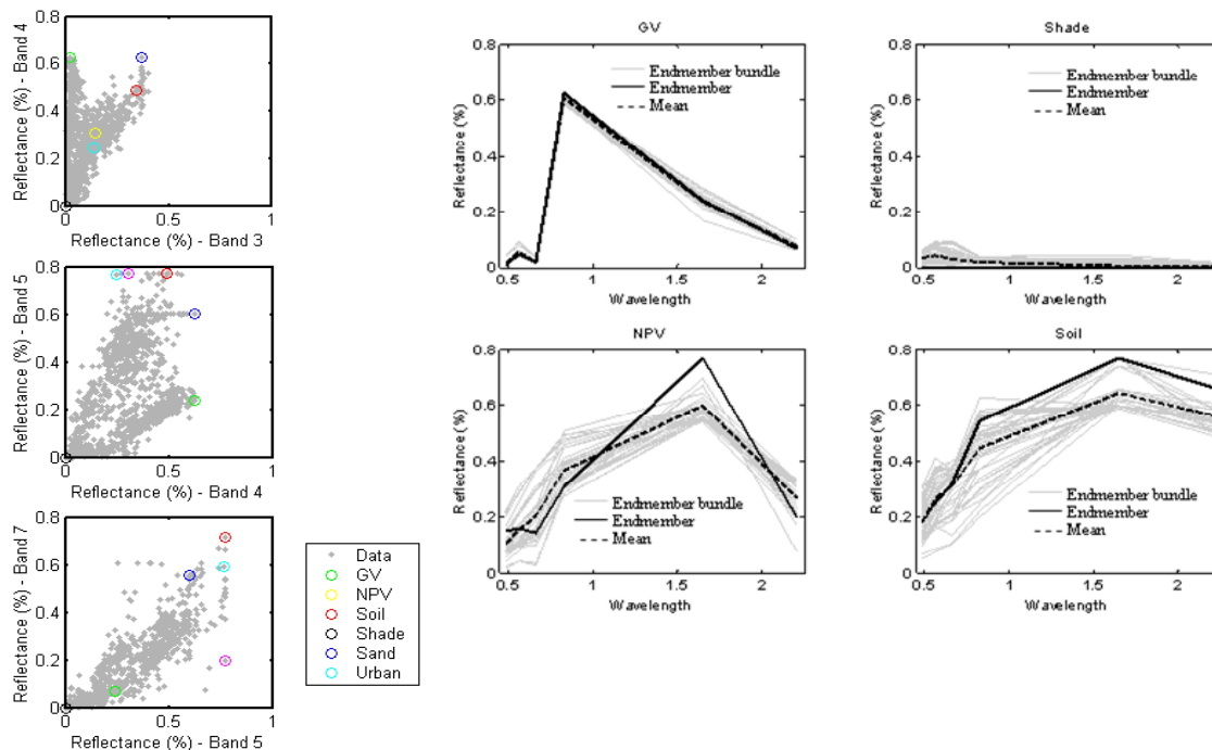
Fig. 3. Image scatter-plots of Landsat bands in reflectance space and the spectral curves of GV, Shade, NPV and Soil (source: Souza Jr. et al., 2005).
