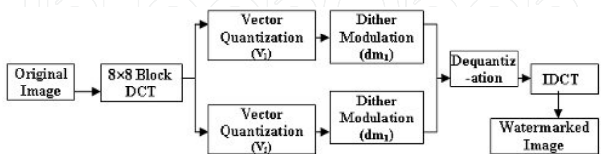
Fig. 13. Watermark Embedding
