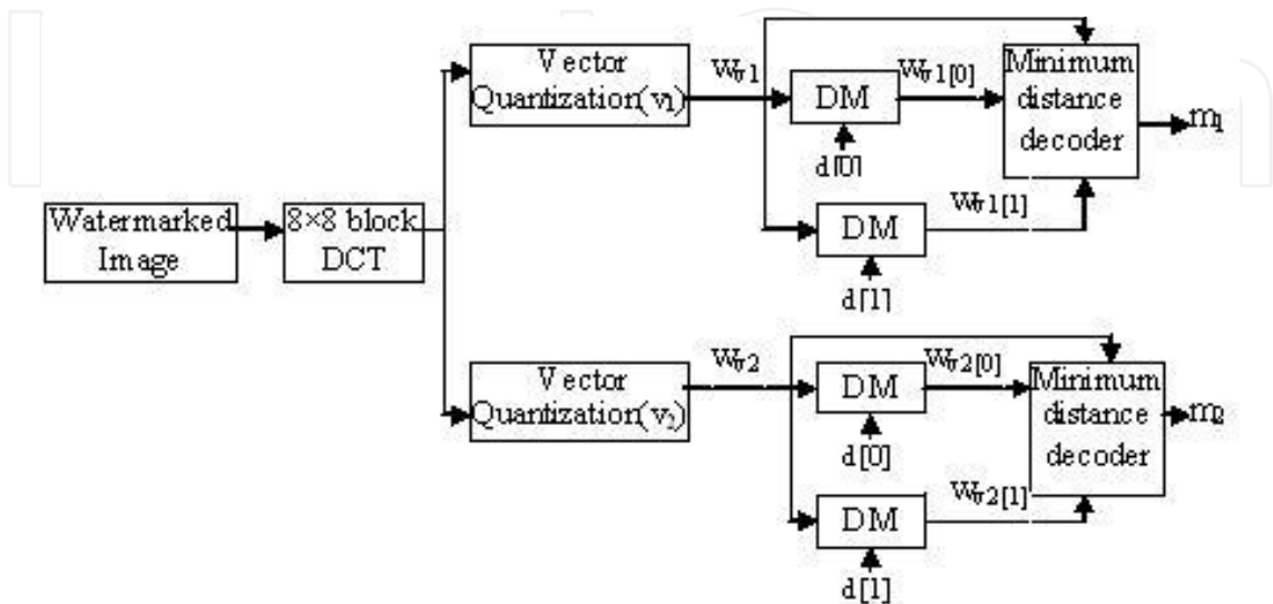
Fig. 15. Watermark extraction
