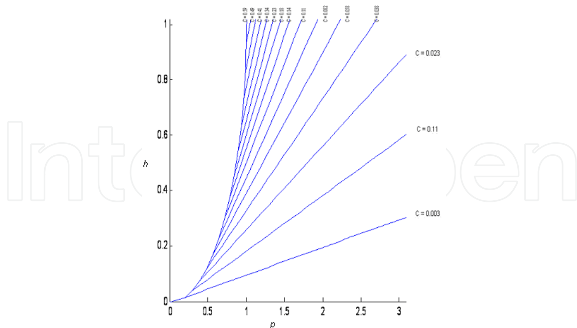
Fig. 9. Relation between thread spacing and crimp height
