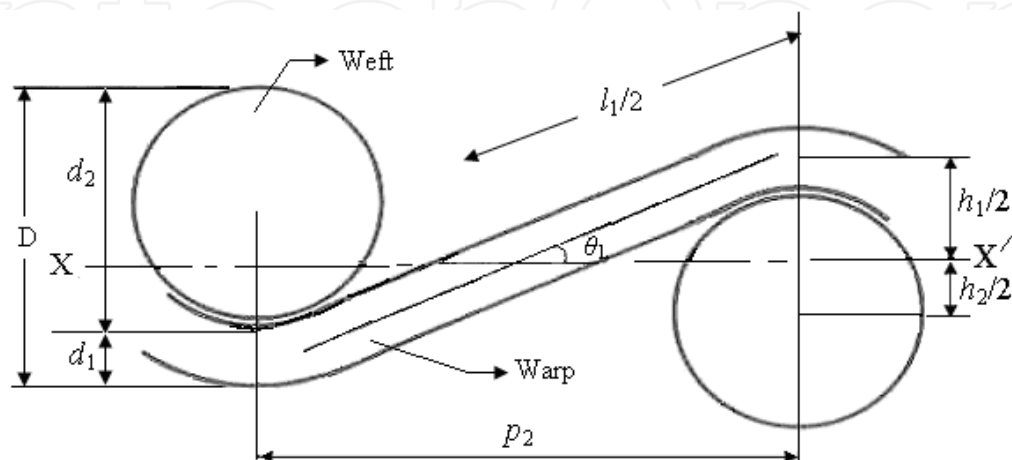
Fig. 5. Peirce's model of plain weave
