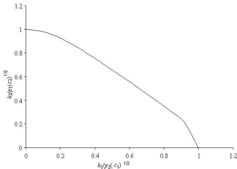
Fig. 11. Relation between warp and weft crimp in jammed fabric
