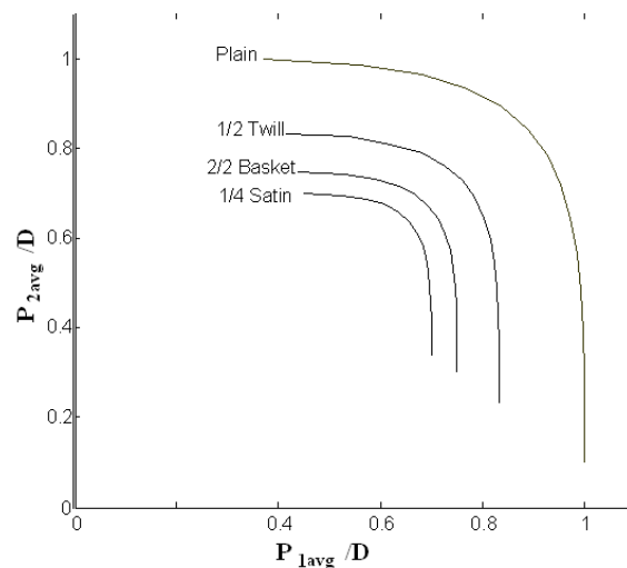
Fig. 6. Relation between average thread spacing in warp and weft for different weaves (Circular cross-section, yarn tex=30, \varnothing=0.6 , \rho=1.52 )
