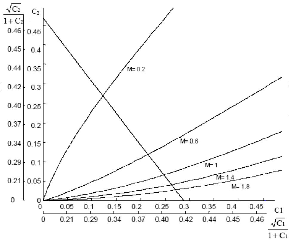
Fig. 19. Interaction of crimp interchange and crimp balance equations ( l_1/D > l_2/D )
