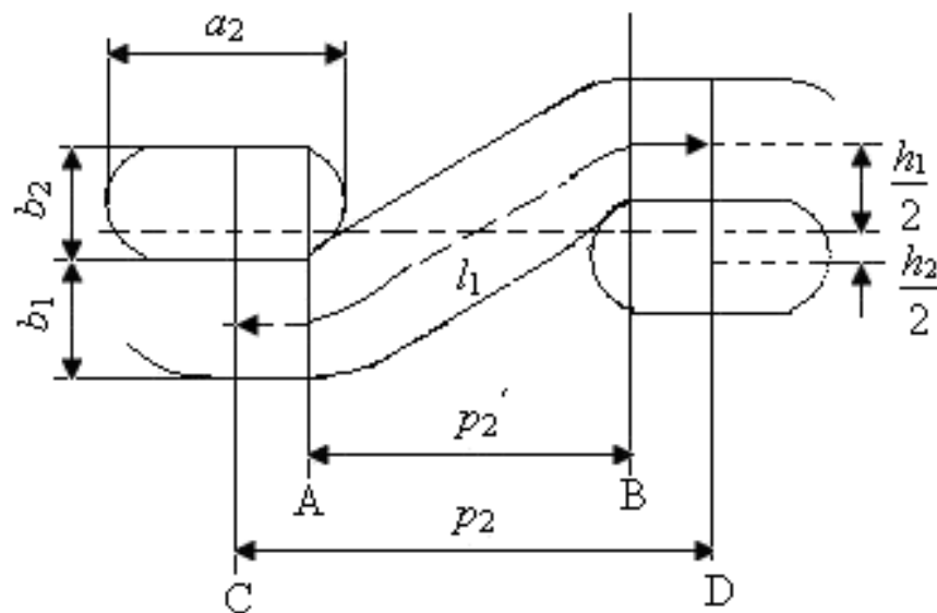
Fig. 8. Race track cross-section
