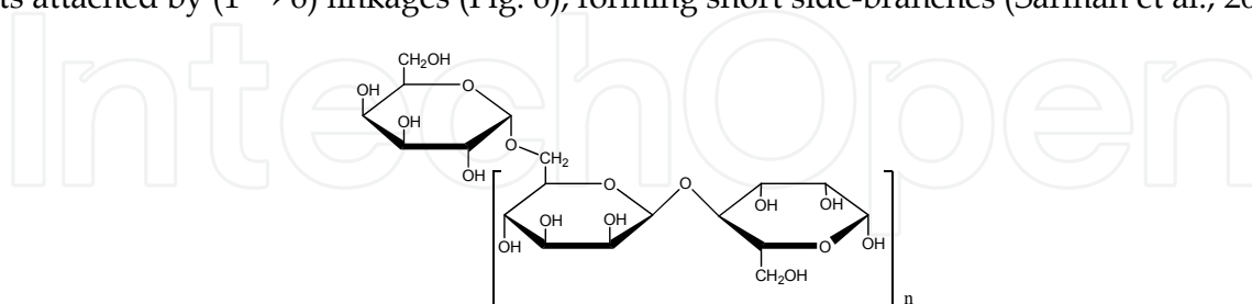
Fig. 6. Chemical structure of guar gum.
