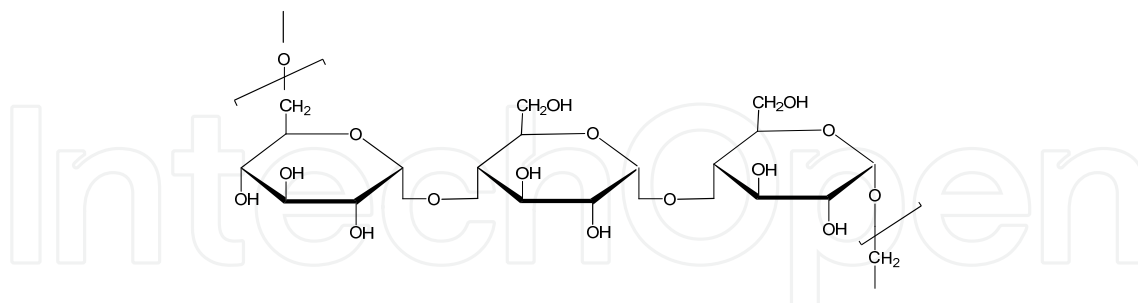
Fig. 5. Chemical structure of pullulan.
