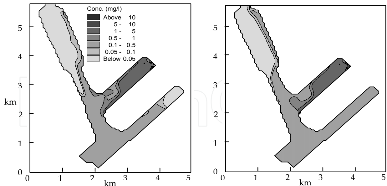
Fig. 4. Concentration map after 2 yrs (left), and 7 yrs (right) from start of simulation with a continuous loading rate of 1.0 g/s at St2.
