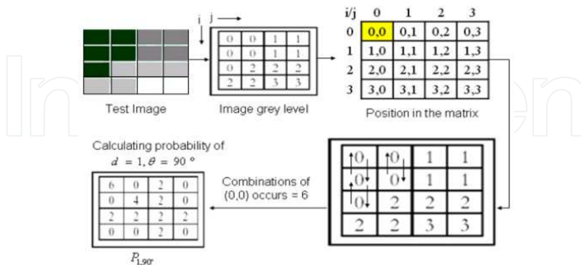
Fig. 6. Constructing SGLCM spatial matrix based on \theta=90^\circ, d=1 , using 4 \times 4 ROI block. A reference pixel of 0 and its neighbour of 0 at the direction of 90^\circ will contribute one count to the matrix element (0,0). Similar to Fig. 4, a reference pixel of 3 and its vertical neighbour of 2 would contribute one count to the matrix element (3,2) and one count to the matrix element (2,3).
