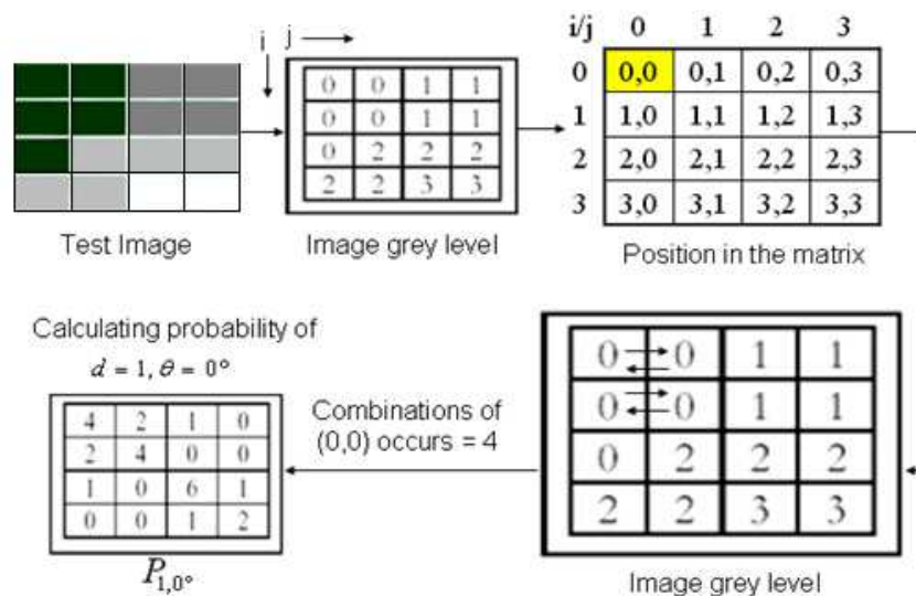
Fig. 5. Constructing SGLCM spatial matrix based on \theta = 0^\circ , d=1 , using 4 x 4 ROI block. Each pixel within the test image becomes the reference pixel of the position in the matrix of the direction of 0^\circ . A reference pixel of 3 and its horizontal neighbour of 2 would contribute one count to the matrix element (3,2) and one count to the matrix element (2,3).
