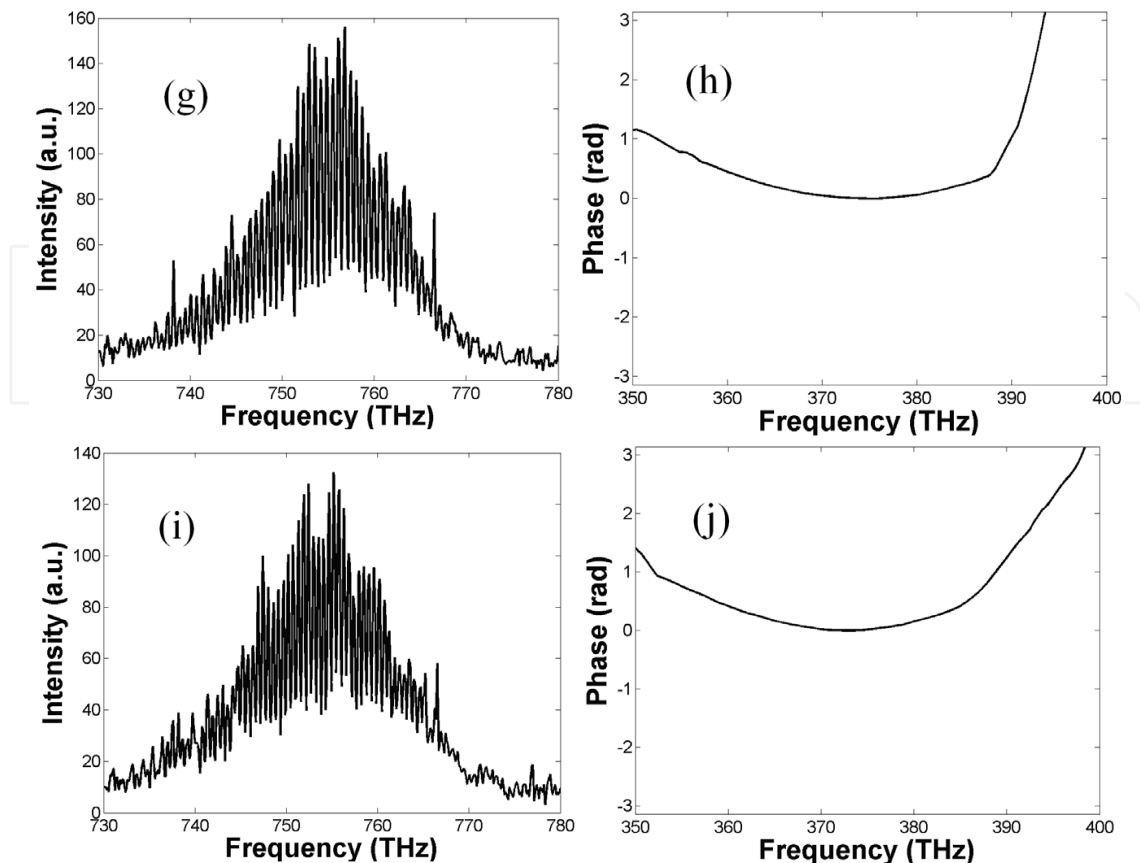
Fig. 7. Measured spectral interferograms with different replicas separations and retrieved spectral phases from the interferograms. (a), (c), (e), (g), and (i) are measured interferograms with replicas separations of 0.22 ps, 0.55 ps, 0.83 ps, 1.58 ps, and 1.82 ps respectively; (b), (d), (f), (h), and (j) are the retrieved spectral phases from interferograms in (a), (c), (e), (g), and (i) respectively.
