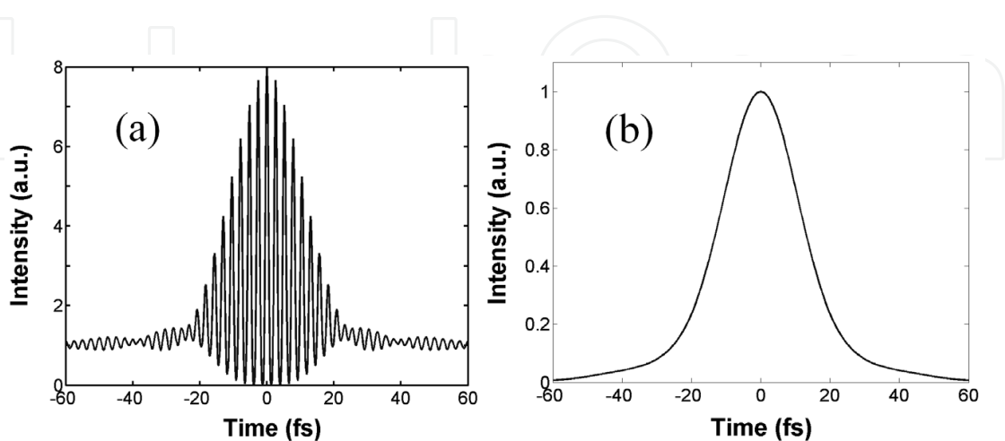
Fig. 6. Simulated autocorrelation traces with reconstructed pulse electric field. (a) Interferometric autocorrelation, (b) intensity autocorrelation.
