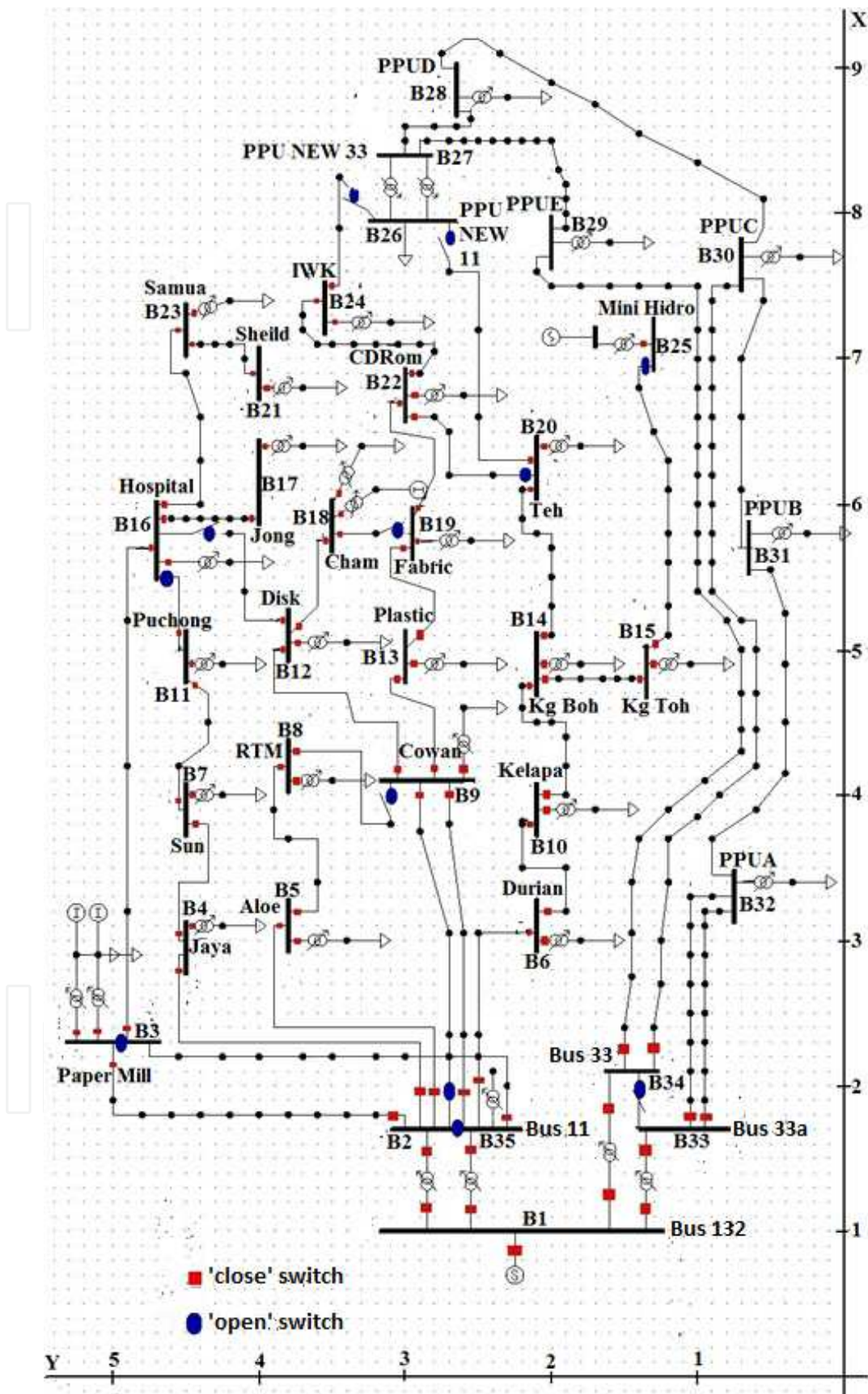
Fig. 13. A single line diagram of 47 buses practical system
