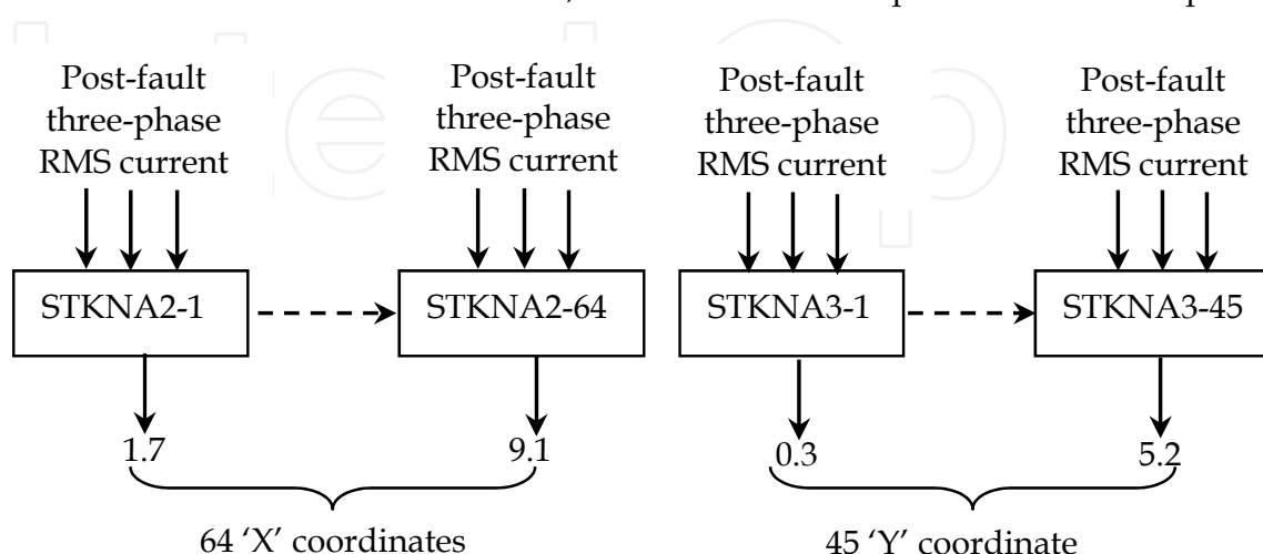
Fig. 11. ANFIS2 and ANFIS3 design for identifying fault location in a 47 buses practical system
