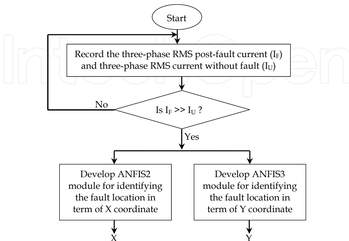
Fig. 10. A procedure for identifying fault location
