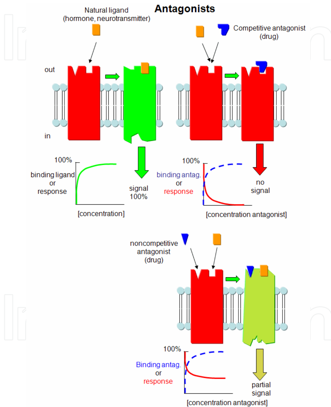
Fig. 17. Sketch is shown for membrane receptor binding with ligand (acting as agonist) and antagonist (acting as inhibitor) in competition with agonist to bind with enzyme. Reproduced with permission [Jakobowski 2010a]
