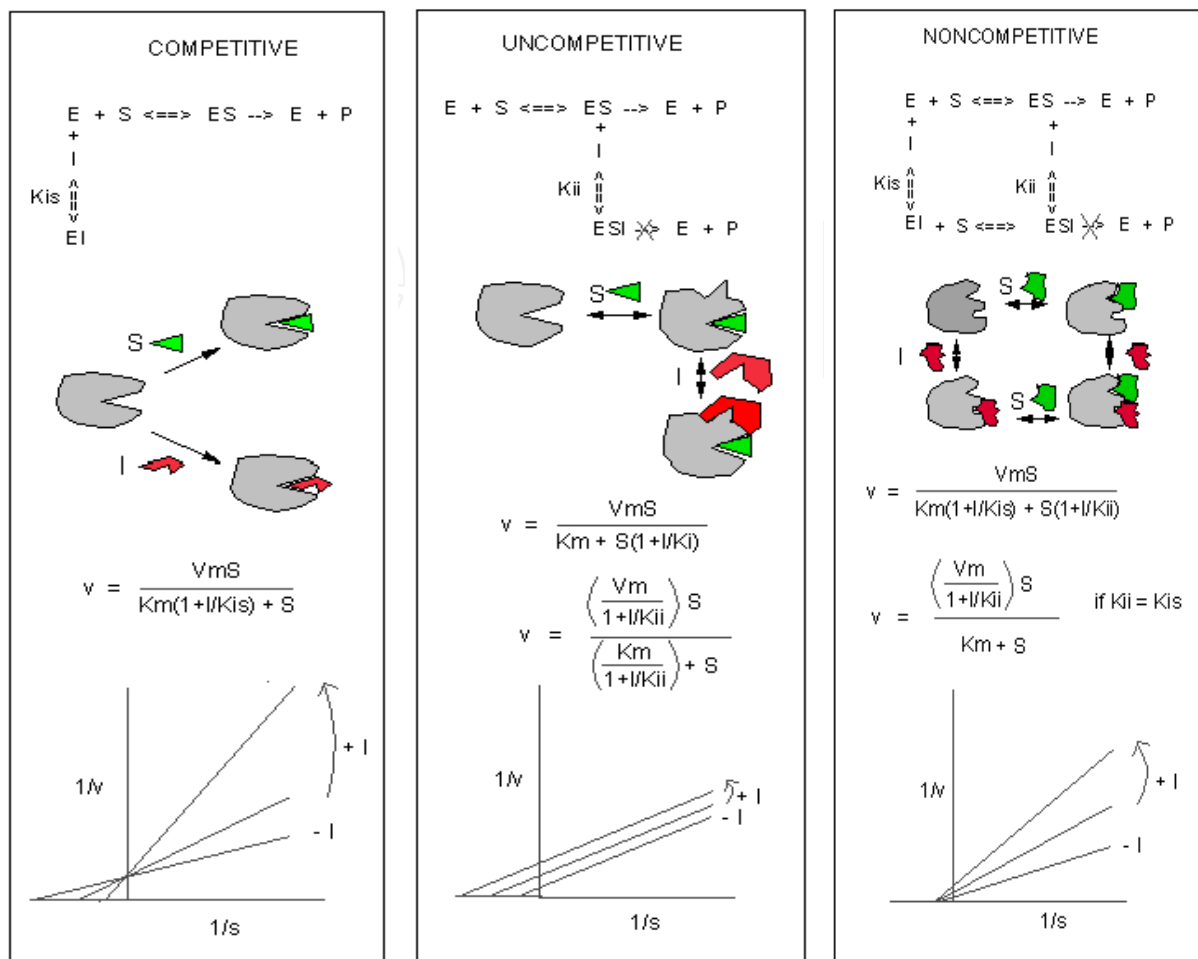
Fig. 15. Sketch of three different enzyme inhibition by competitive, uncompetitive and noncompetitive types are shown with illustration of enzyme-substrate or inhibitor binding, kinetics and graphs.
