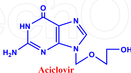
Fig. 5. Aciclovir; the prodrug for the suicidal irreversible inhibition of the viral DNA polymerase.
