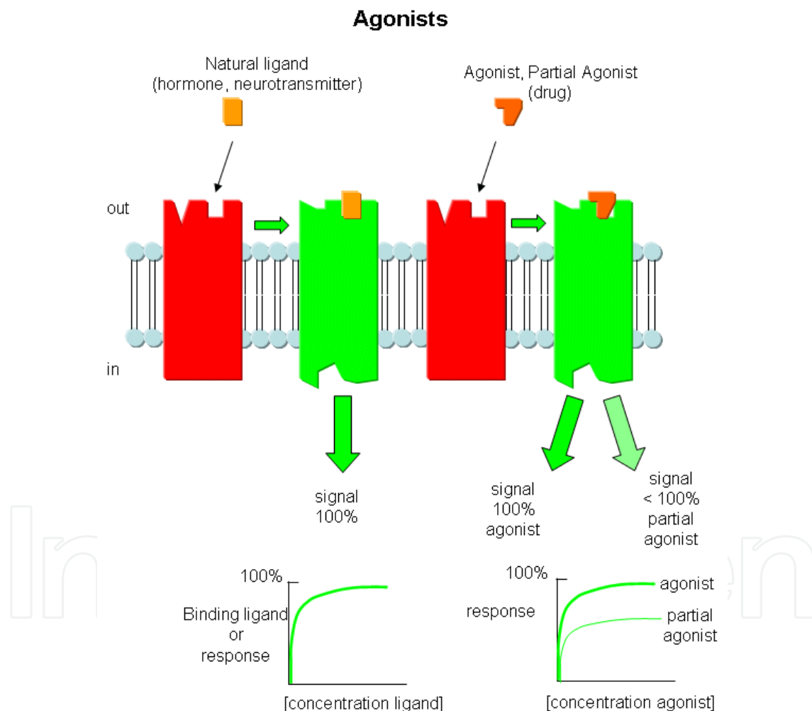
Fig. 16. A sketch is shown for membrane receptor binding with ligand (agonist) acting like as enzyme. Reproduced with permission [Jakobowski 2010a].
