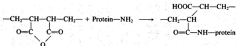
Fig. 21. Scheme of immobilization of enzyme is shown with chemical groups involved in binding of enzyme on solid surface. Reproduced with permission from reference Lieder et al.1980.
