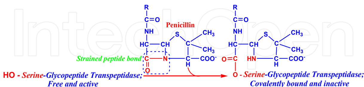
Fig. 6. The suicidal irreversible mechanism-based inhibition of the bacterial enzyme glycopeptide transpeptidase by the antibiotic penicillin.
