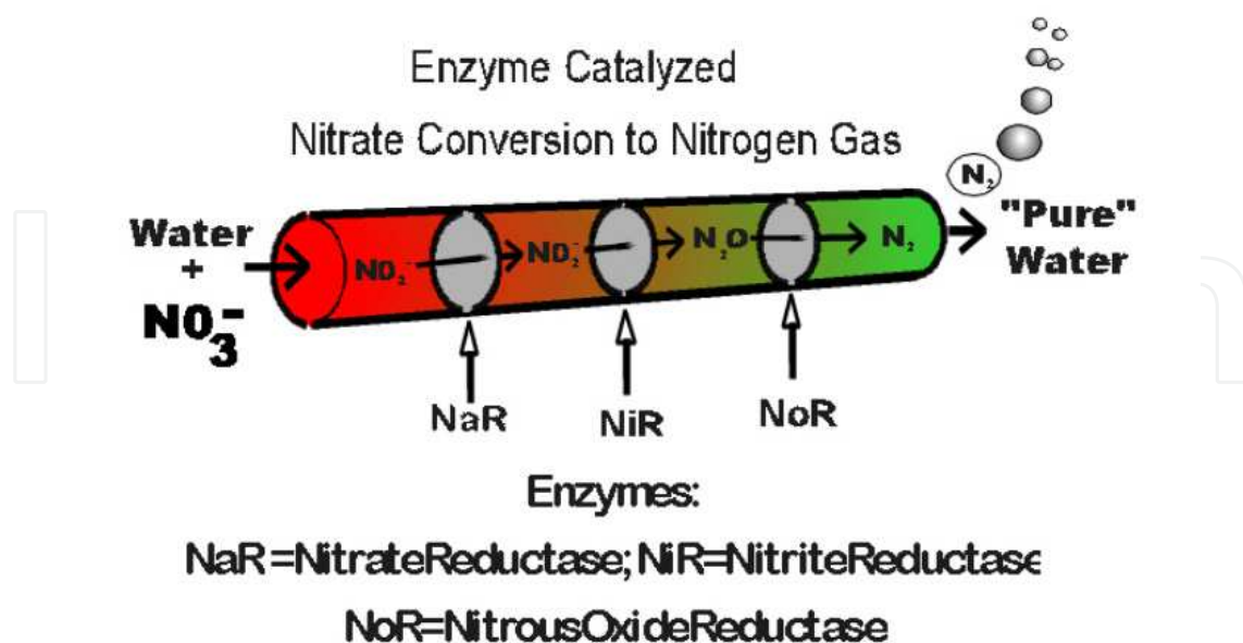
Fig. 28. EzNET® system shows immobilized enzyme on “beads” with an electron-carrying dye. In this system, reduction of nitrate generates environmentally safe nitrogen gas driven by a low voltage direct current. Source: The Nitrate Elimination Co., Inc. 2000.
