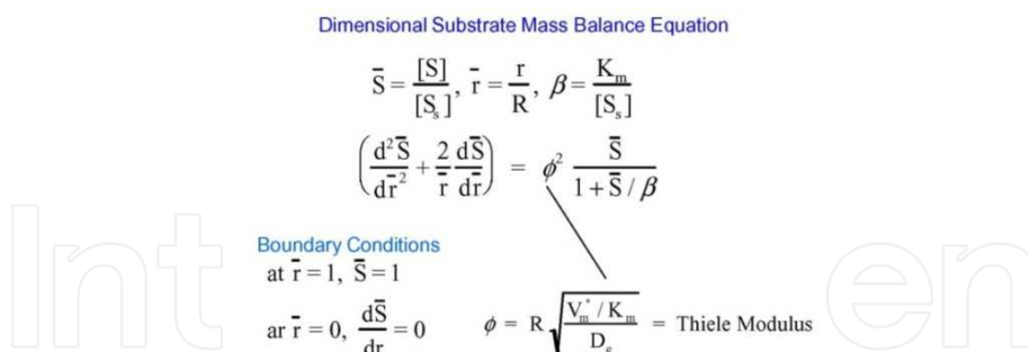
Fig. 23. A scheme of substrate mass balance is shown to calculate S with boundary conditions.
