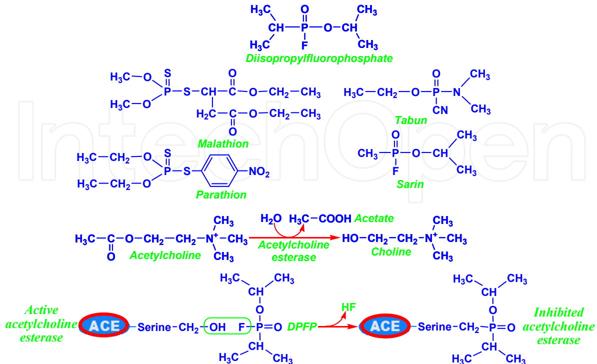
Fig. 2. Organophosphorus compounds and the suicidal irreversible mechanism-based inhibition of the enzyme acetylcholinesterase by diisopropylfluorophosphate. Malathion and parathion are organophosphorus insecticides. The nerve gases Tabun and Sarin are other organophosphorus compounds.
