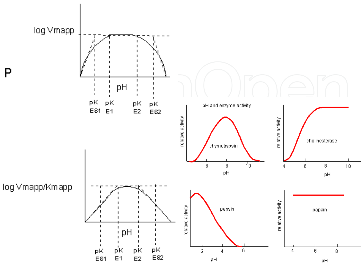
Fig. 20. Graphs of different pH effects on enzyme catalyzed reactions as \log V_m(app) and V_m/K_m(app) are shown on left. Different enzymes such as chymotrypsin, cholinesterase, pepsin and papain are illustrated with different rates of enzyme reaction. Reproduced with permission [Jakobowski 2010a]
