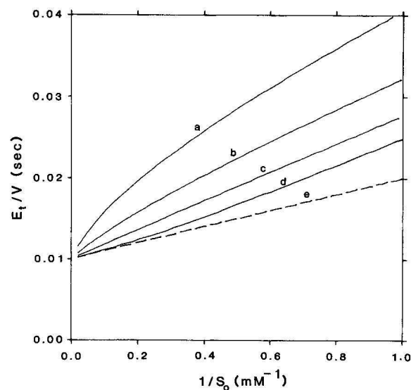
Fig. 24. Effect of one or more inhibitor molecules on enzyme kinetics and their inhibition effect dependent on 1/S_0 . Reproduced with permission from Rees et al. 1984.
