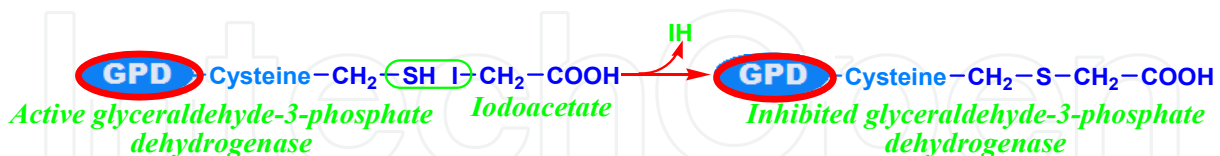
Fig. 3. The suicidal irreversible mechanism-based inhibition of the enzyme glyceraldehyde-3-phosphate dehydrogenase by iodoacetate.
