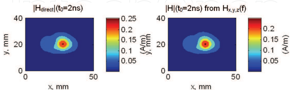
Fig. 9. Comparison of H-field maps modulus |H|(t_0 = 2 \text{ ns}) obtained from the direct formulae (in left) and from the time-frequency computation method proposed for z_0 = 6.5 mm
