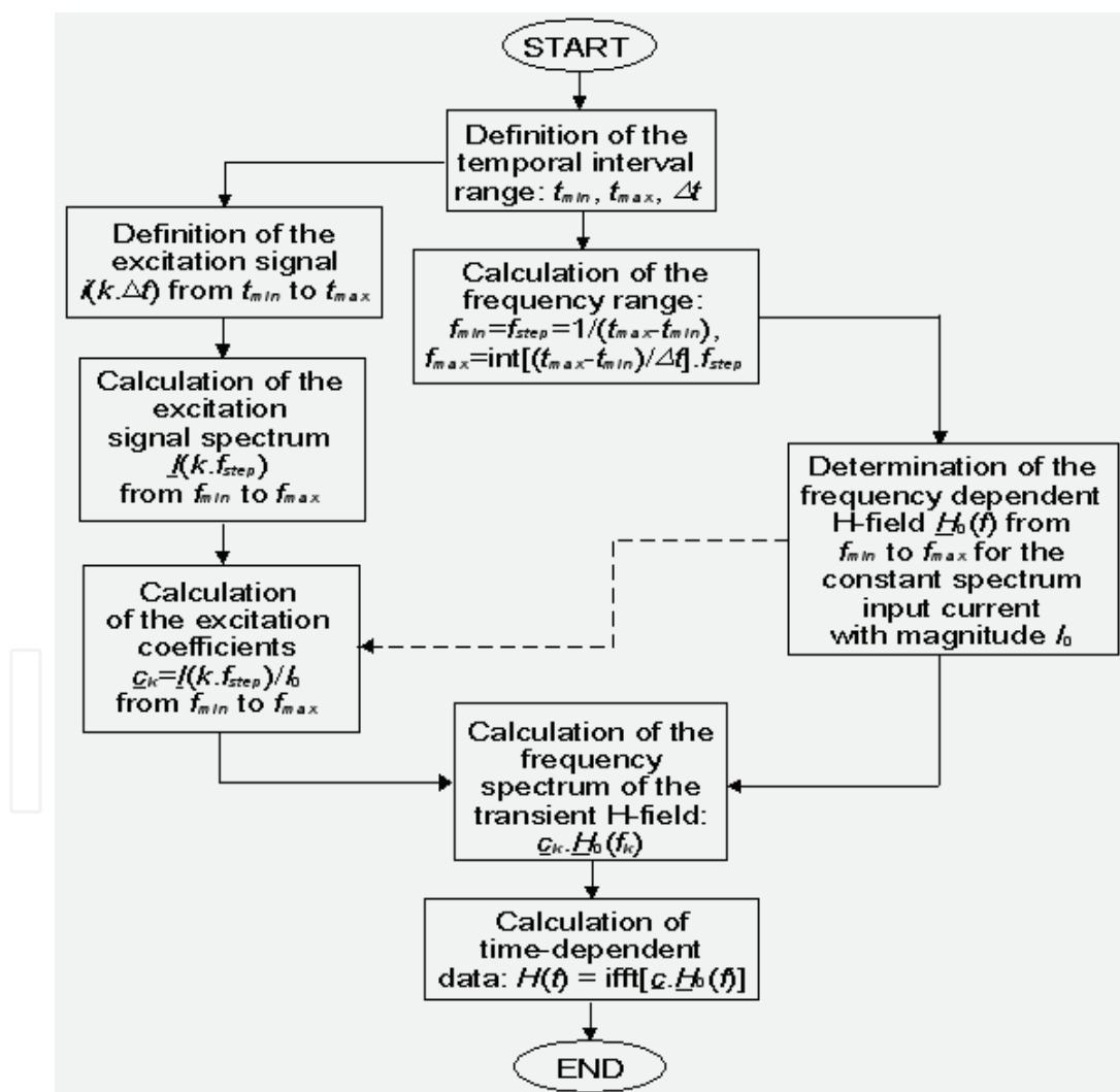
Fig. 2. Flow work illustrating the transient H-field radiation computation-method proposed knowing the temporal range, t_{min} and t_{max} step \Delta t of the excitation signal i(t_k) and also the frequency-dependent H-field \underline{H}_0(f) (here the under bar indicates the complex variables)
