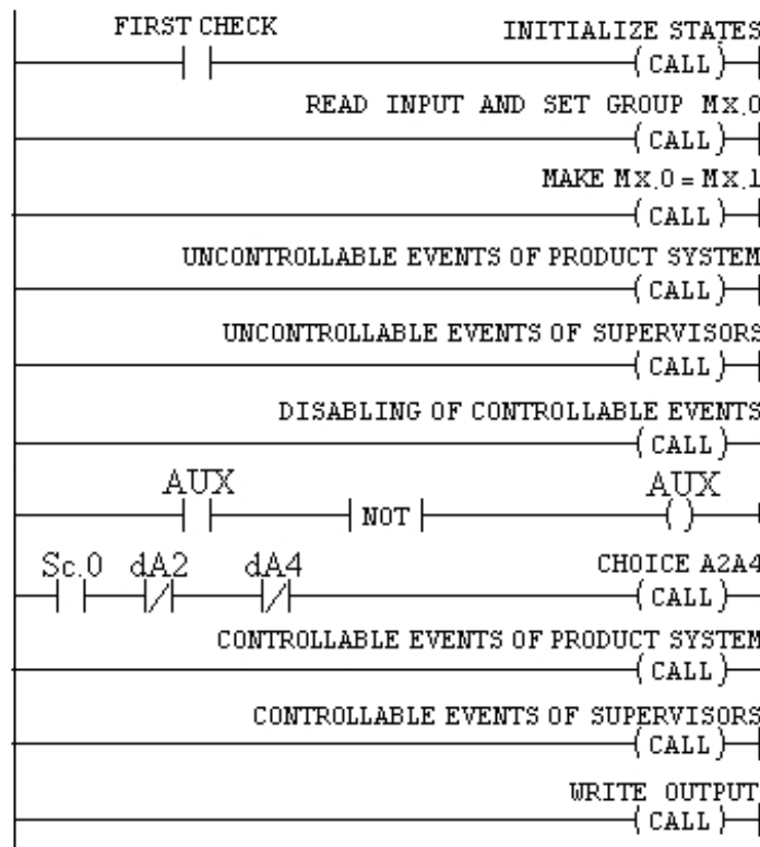
Fig. 11. DECON9 main routine
