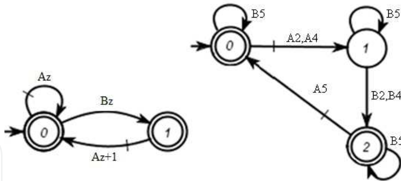
Fig. 10. Reduced supervisors automata
