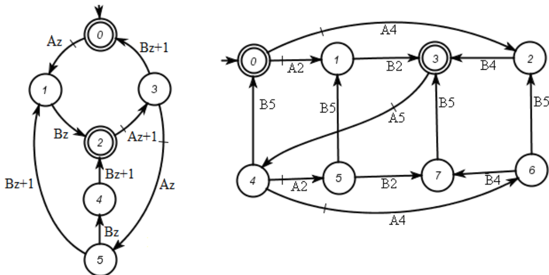
Fig. 9. Local modular supervisors
