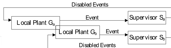
Fig. 2. Local modular supervisory control architecture (Queiroz & Cury, 2002)
