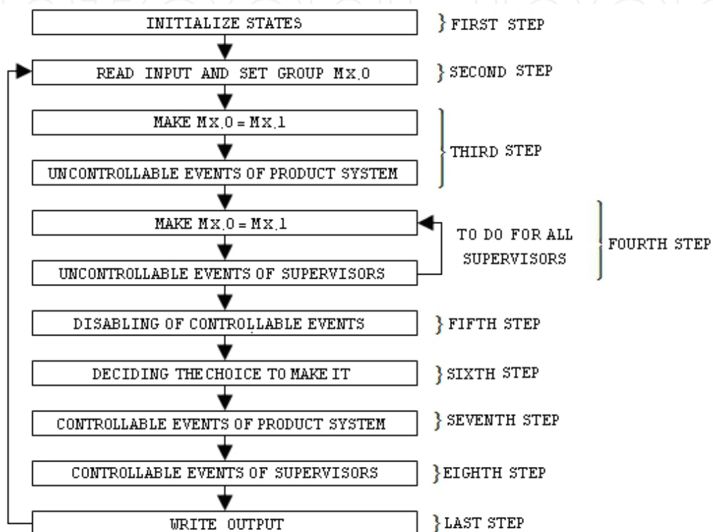
Fig. 5. Complete flowchart of the main routine
