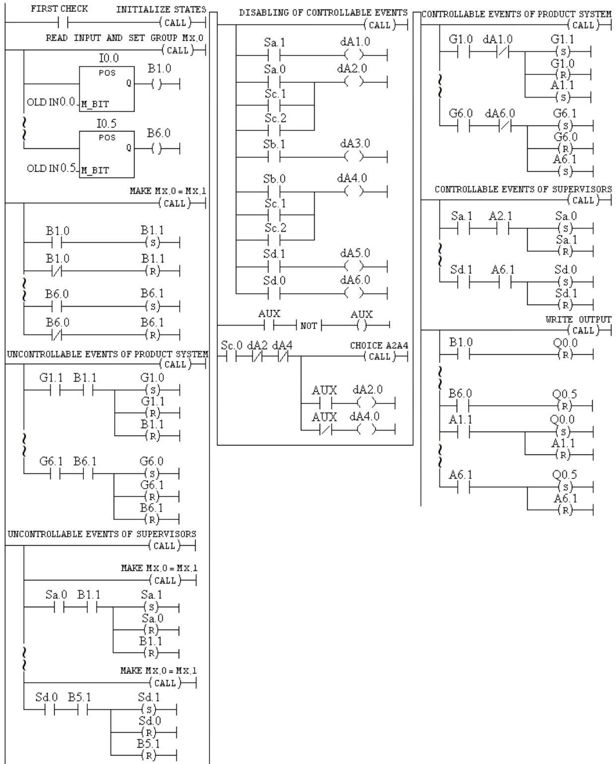
Fig. 12. PLC implementation for the case study
