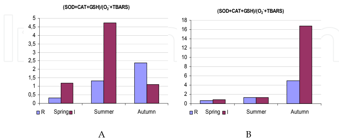
Fig. 3. Integrated Oxidative Stress index of liver (A) and gills (B) of common carp from relatively clean (R) and chronically polluted (I) field sites in three seasons, calculated from their SOD and catalase activities, GSH level, superoxide anion production and TBARS levels (from Falfushynska et al., 2009 with permission).
