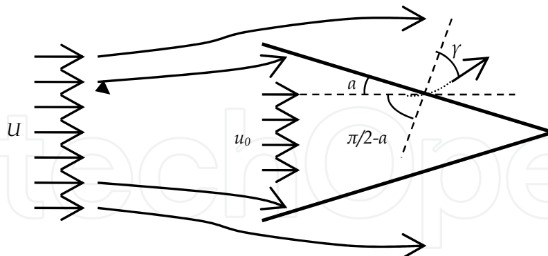
Fig. 2. Sketch of flow through a conical net with taper angle \alpha and filtration efficiency F = u_0/U , the angle \gamma describes streamline deflection through the net wall ("cf." from Gjørund and Enerhaug, 2010).
