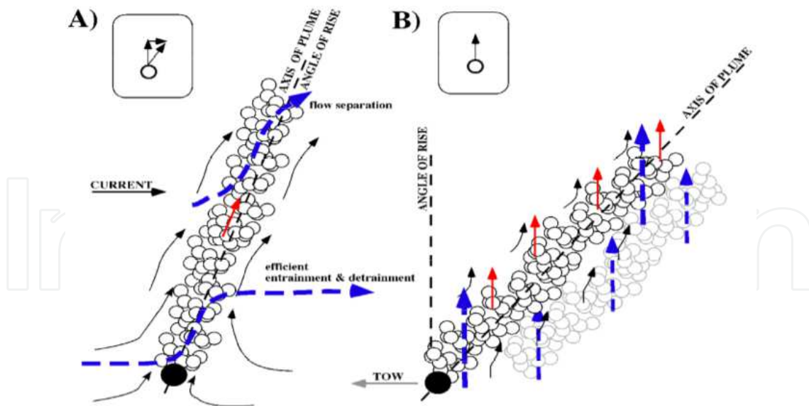
Fig. 6. Two dimensional schematic of a bubble plume for A) a fixed bubble source in a uniform horizontal current and B) towed bubble source through quiescent water. Inset shows details of individual bubble motions. Red and black arrows pertain to bubbles and entrained water, respectively. Grayed bubbles represent plume several seconds earlier, and remnant, persistent fluid motions.
