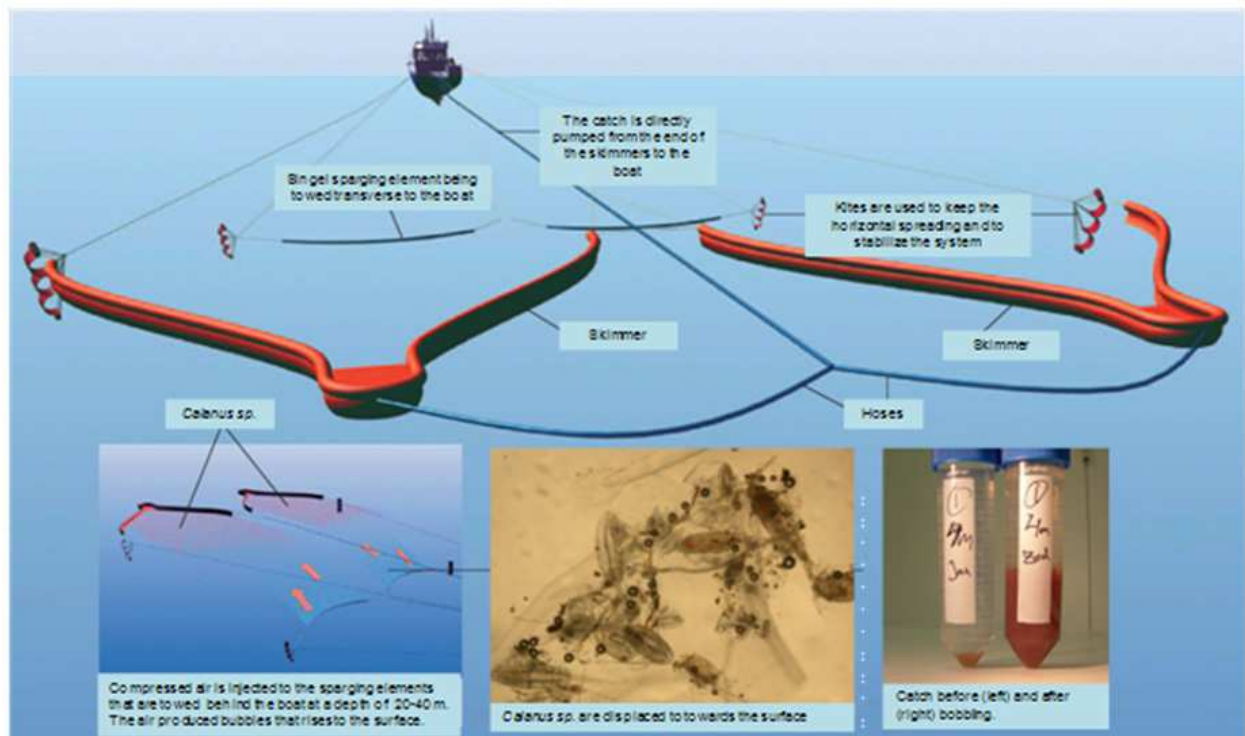
Fig. 4. Initial prototype of a skimmer trawl for commercial harvesting of Calanus sp. Air is released from a single perforated hose at 20-40 m depth to produce small bubbles. These bubbles while rising displace Calanus sp. towards the surface. Here they are collected by skimmer and directly pumped to the boat. Animation: Mats Heide, SINTEF.
