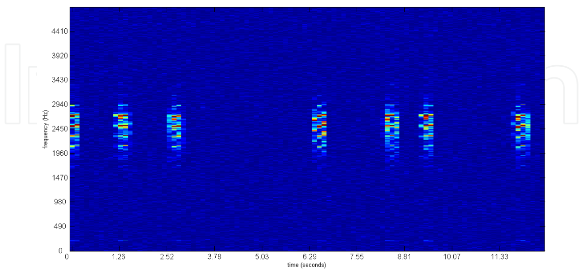
Fig. 5. The 2D spectrogram corresponding to the frog vocalization in Fig. 4.
