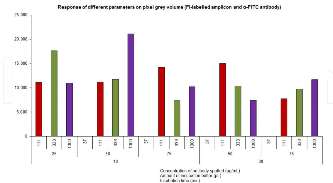
Fig. 10. Influence of the \alpha -FL antibody concentration (37, 111, 333, or 1000 \mu g mL -1 ); conditions as described under Figure 9 except for the amplicon: 1 \mu L of the amplicon of Listeria 16S RNA labelled with biotin and fluorescein.
