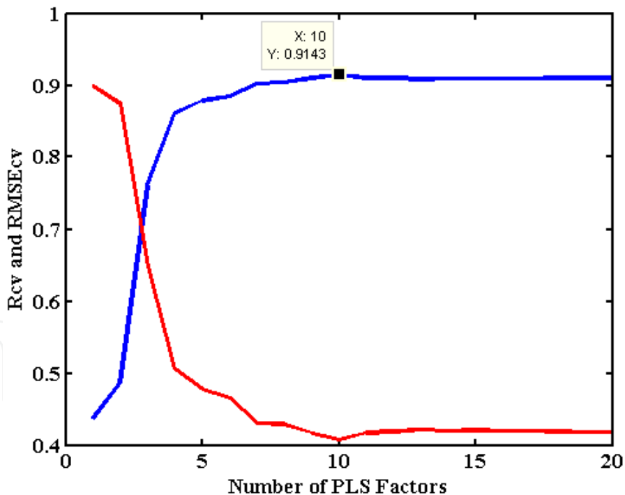
Fig. 4. Optimal PC number of prediction model for filter-paper samples.
