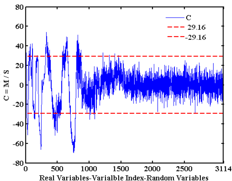
Fig. 5. Variables selected by UVE.
