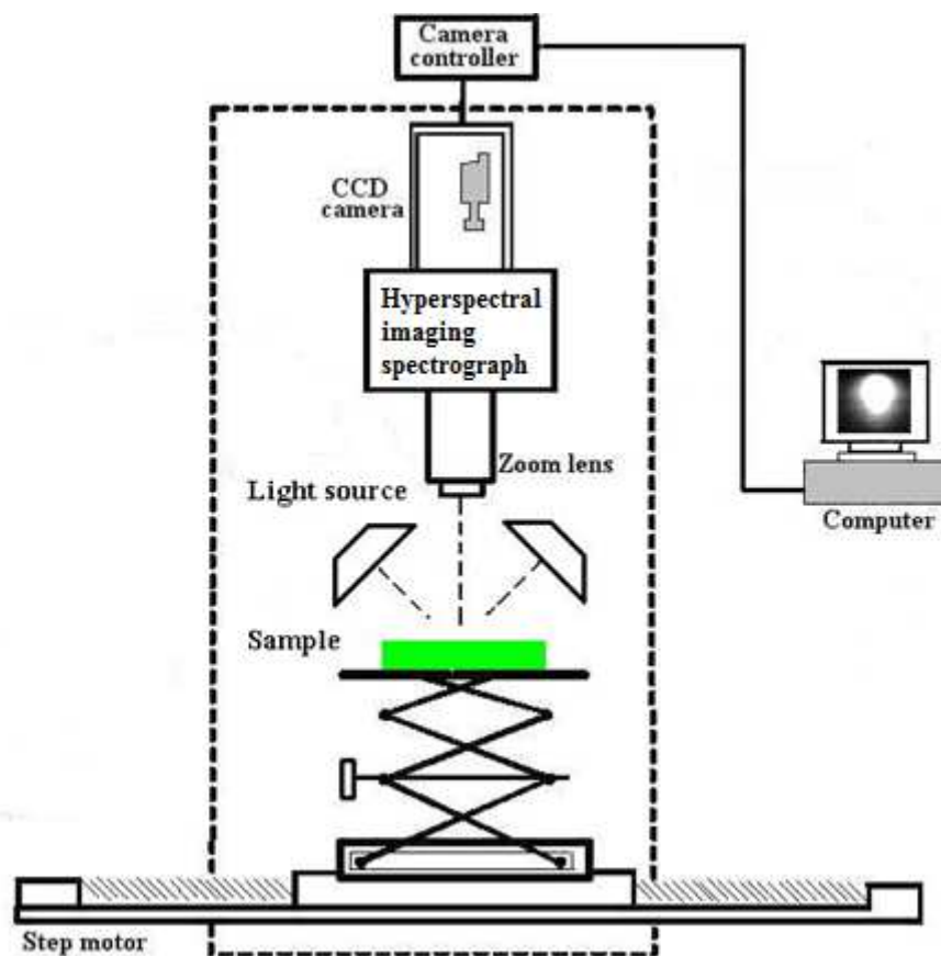
Fig. 7. Hyperspectral fluorescence imaging system.
