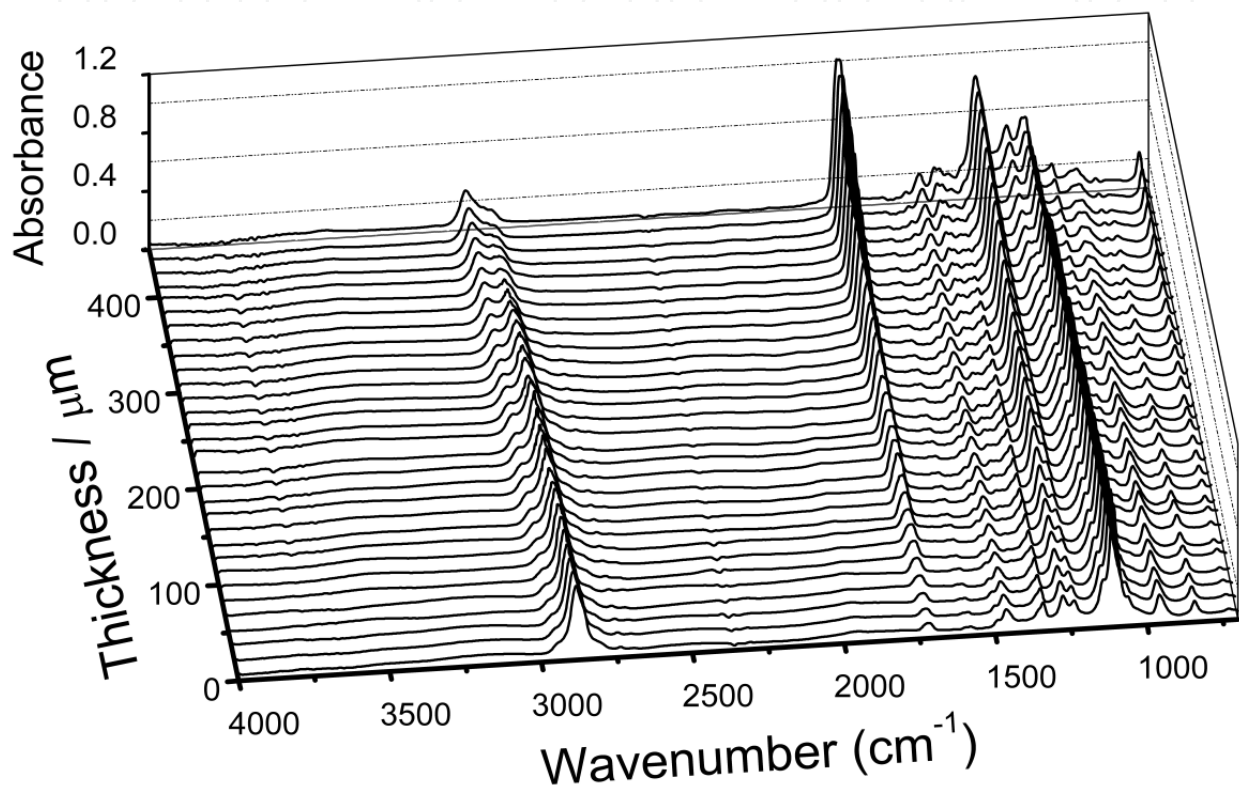
Fig. 7. Results of FT-IR mapping measurements on the cross section along the direction vertical to the sample surface.
