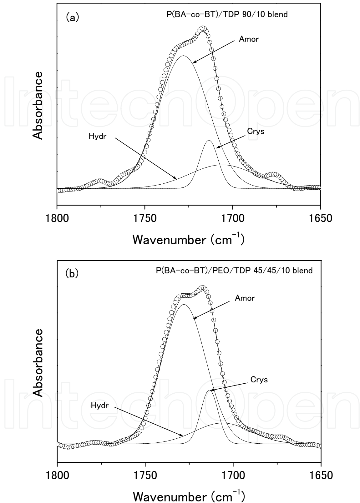
Fig. 3. Infrared spectra in the carbonyl stretching region for binary P(BA-co-BT)/TDP=90/10 blend (a) and ternary P(BA-co-BT)/PEO/TDP=45/45/10 blend (b) resolved by curve-fitting program; Amor.: amorphous component; Crys.: crystalline component; Hydr.: hydrogen-bonded component; Fitt.: curve-fitted; Exp.: experimental spectrum.
