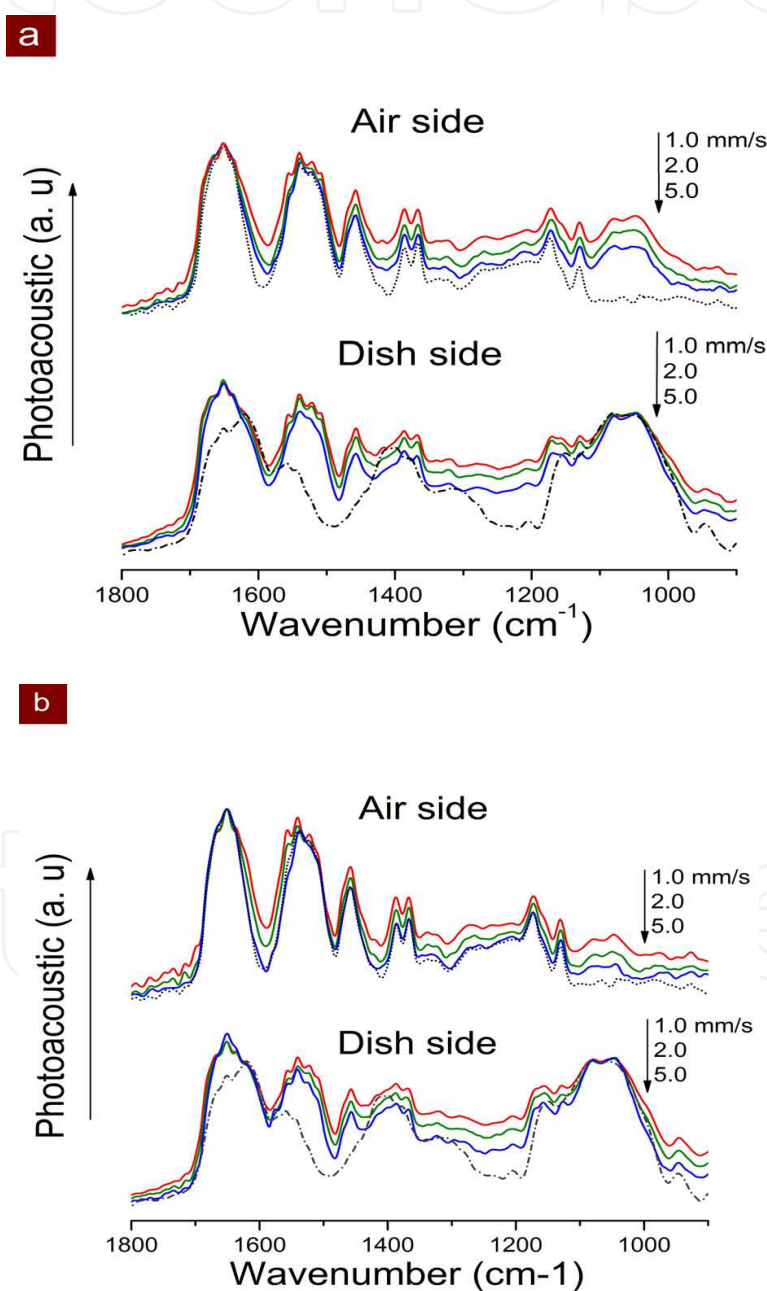
Fig. 8. Results of PAS-FTIR spectroscopy measurements on the films cast on NTPSD and PTPSD in vacuum condition.
