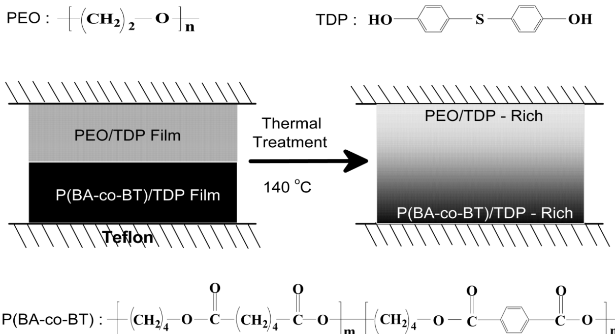
Fig. 4. Schematic illustration of the formation of P(BA-co-BT)/PEO/TDP compositional gradient film.
