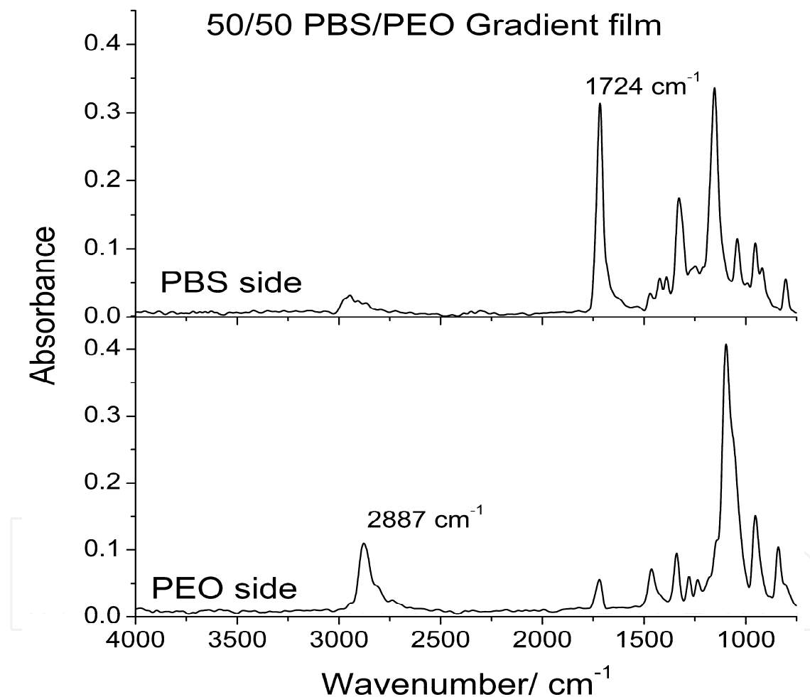
Fig. 2. ATR-FTIR spectra on both surfaces of the compositional gradient film observed at room temperature.
