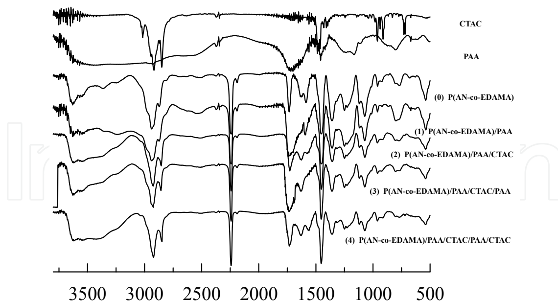
Fig. 3-1. FT-IR spectra of base membrane and membrane with self-assembled layers.
