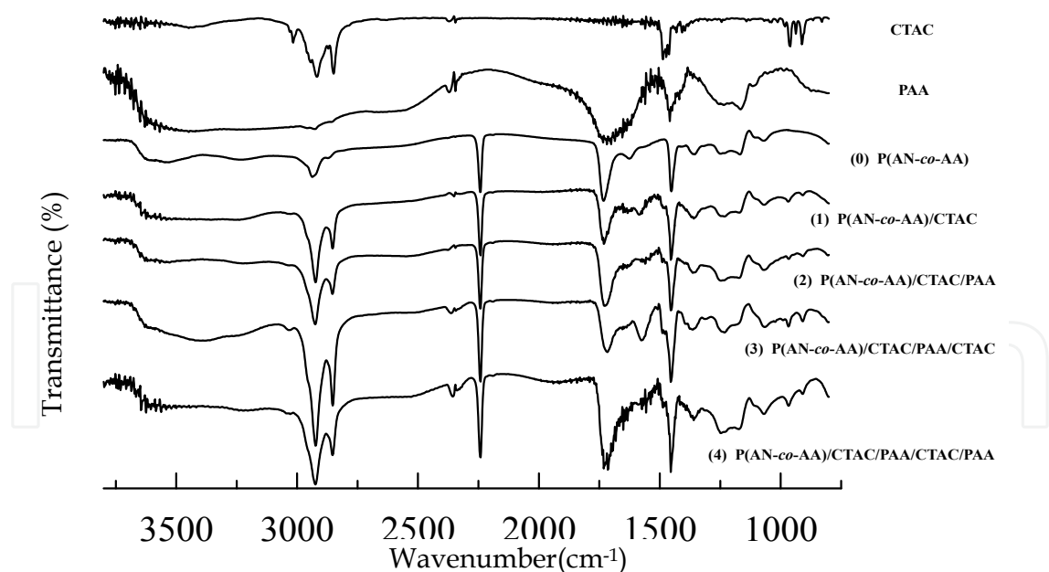
Fig. 2-1. Comparison of FT-IR spectra of the base P(AN-co-AA) and multi-layer composites of CTAC/PAA on the base P(AN-co-AA). The layer number of each spectrum was represented as 0, 1, 2, 3 and 4 for P(AN-co-AA), P(AN-co-AA)/CTAC, P(AN-co-AA)/CTAC/PAA, P(AN-co-AA)/CTAC/PAA/CTAC and P(AN-co-AA)/CTAC/PAA/CTAC/PAA, respectively.
