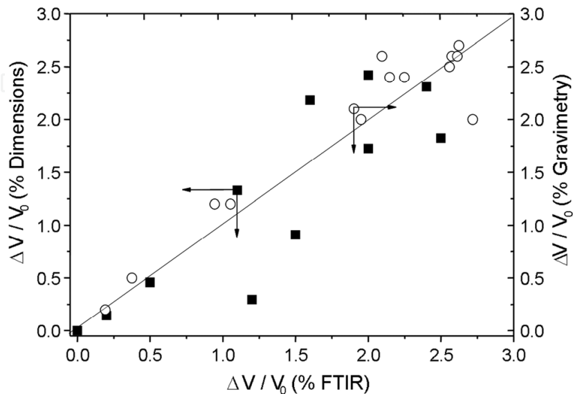
Fig. 13. Comparison of volume change determined by n-FTIR, (\Delta V / V_0)_{IR} , and measured with a micrometer, (left) or by gravimetry (right), for fully cured DGEBA/Poly(aminopropylsiloxane) with 0.381 mm thickness.
