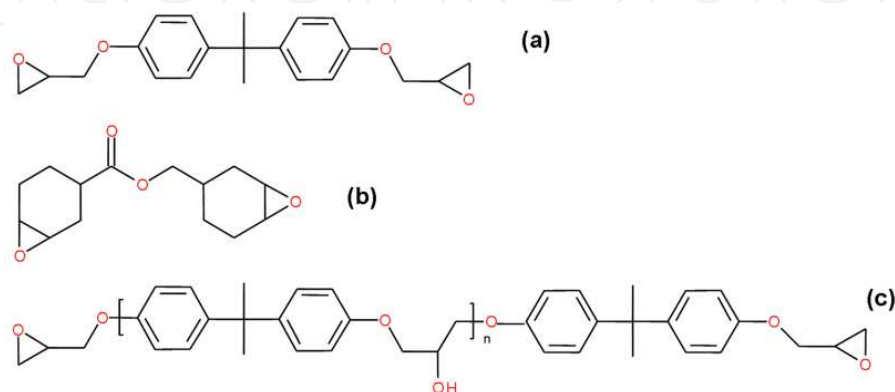
Fig. 2. Chemical structures of common epoxy resins: a) 2,2-Bis[4-(glycidyloxy)phenyl]propane (DGEBA); b) 3,4-Epoxy cyclohexylmethyl-3,4-epoxy cyclohexane carboxylate (ECC); c) DGEBA oligomer, n = 0.2 typically.
