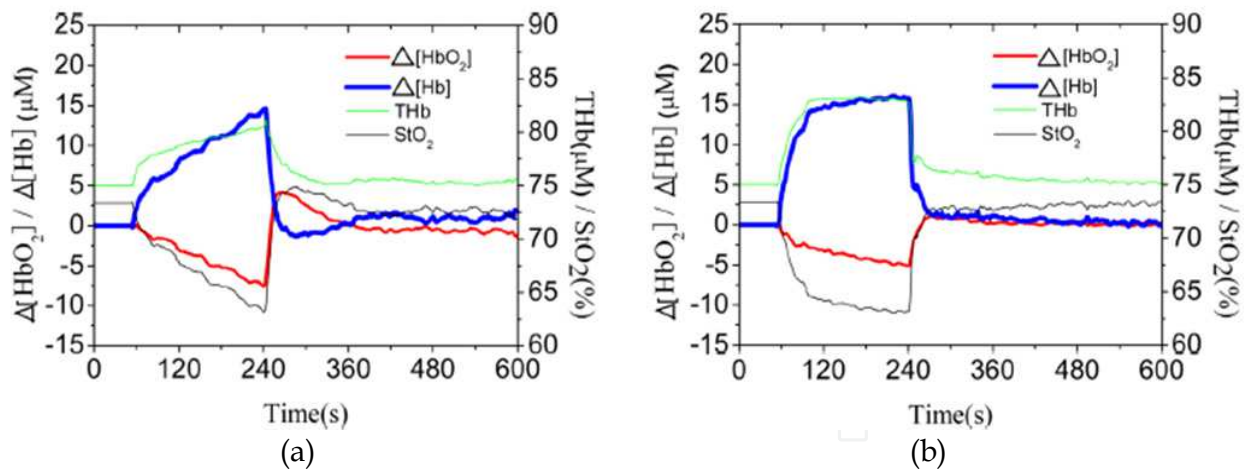
Fig. 6. Temporal tracings of tissue oxygen saturation (StO 2 ), total hemoglobin (THb), oxy-hemoglobin (HbO 2 ) and deoxy-hemoglobin (Hb) response to an AOT assessment: (a) the slower response of oxygenation dynamics, and (b) the faster response of oxygenation dynamics [Wu et al., 2011].
