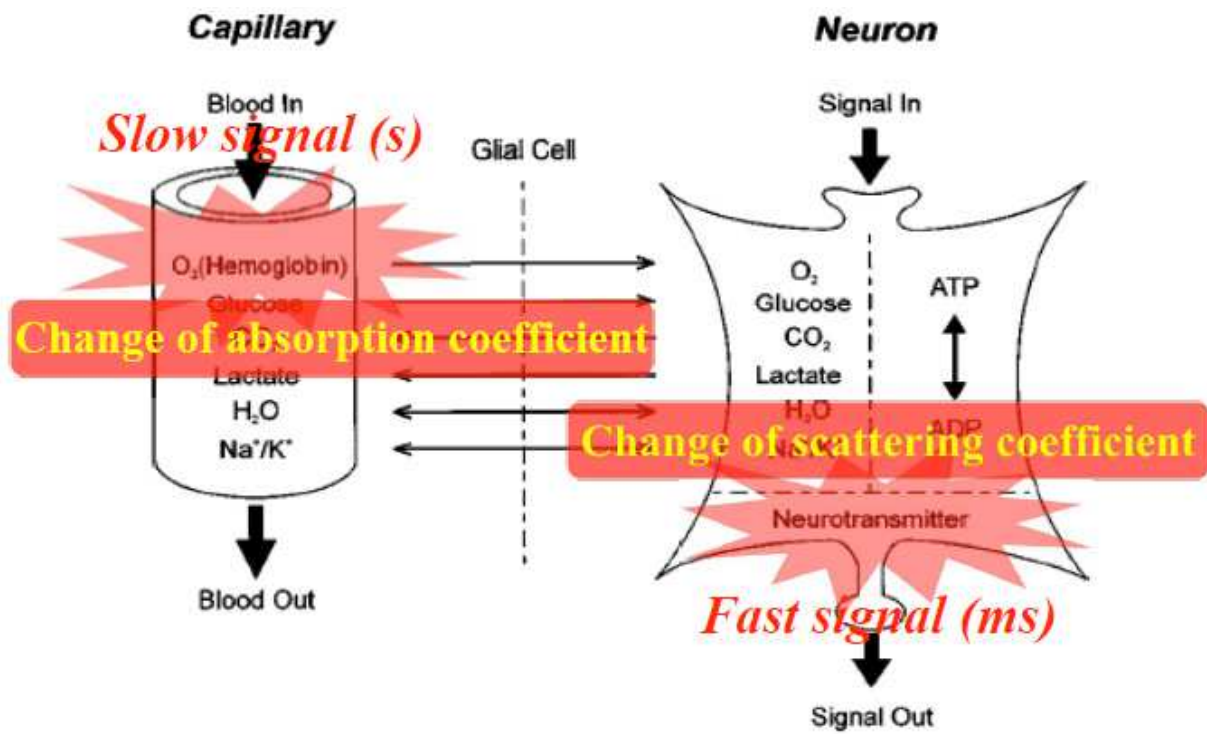
Fig. 8. Neuron-vascular coupling
