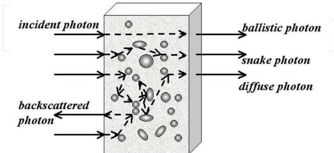
Fig. 2. Illustration of photon migration in a turbid medium.
