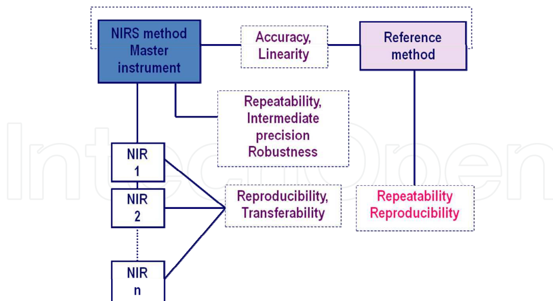
Fig. 3. The validation protocol of the NIRS method as being applied in wheat quality control scanning monochromator Infratec 1241 Grain Analyzer with the ANN calibration model for protein content used in the transmittance mode (FOSS Analytical, Denmark).
