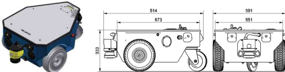
Fig. 13. Neobotix Platform [16]
