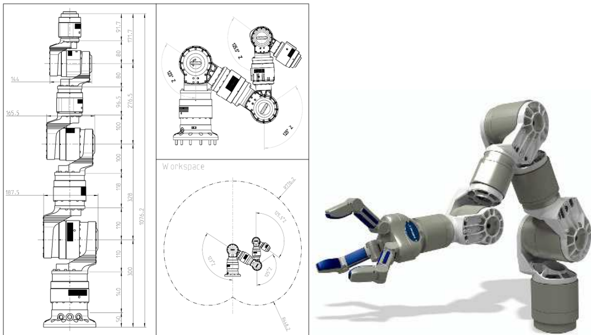
Fig. 12. Schunk robotic arm (a) [16]
