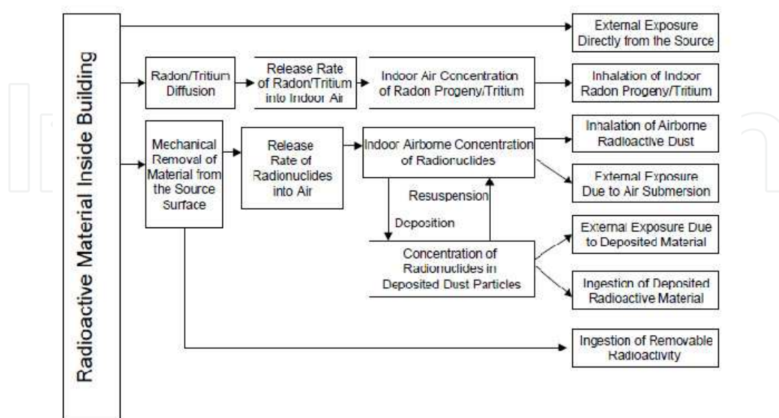
Fig. 6. Exposure Pathways Incorporated into the RESRAD-BUILD Computer Code [9]
