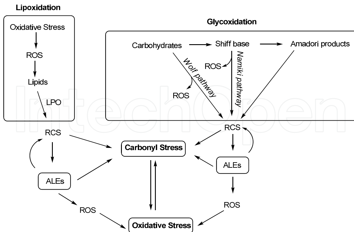
Fig. 15. Relation between lipoxidation, glycooxidation and carbonyl/oxidative stress.
