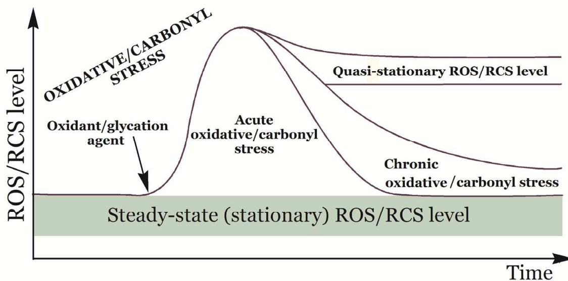
Fig. 14. The dynamics of glycooxidation/lipooxidation-induced perturbations of level of reactive oxygen and carbonyl species in living organisms (modified from (Lushchak, 2011b)).
