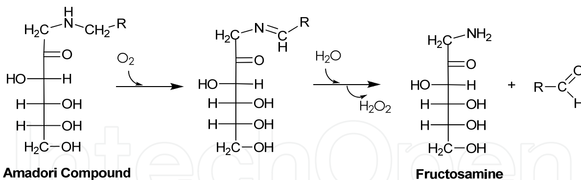
Fig. 18. Degradation of Amadori compound by fructosylamine oxidase.
