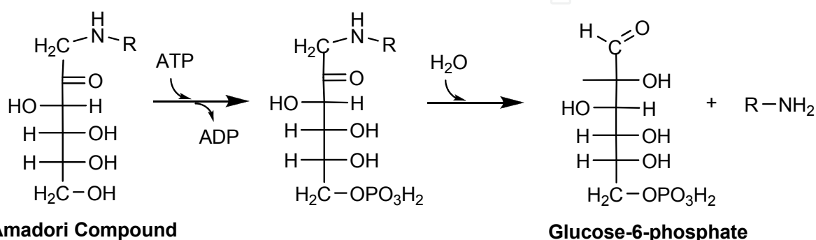
Fig. 19. Degradation of Amadori compound by fructosylamine kinase.
