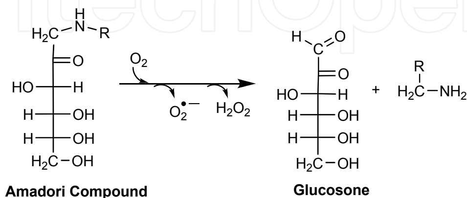
Fig. 7. Formation of glucosone from the Amadori compound.
