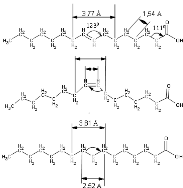
Fig. 1. Structure of different isomers of C16 (Willett, 2006)
