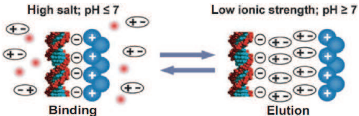
Fig. 2. Interactions between nucleic acids and silica in conditions employed for binding and elution (from Esser et al. , 2006)
