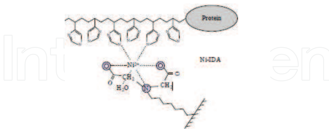
Fig. 8. Model of the interaction between residues in the His tag and the metal ion in tridentate (IDA) IMAC ligand.
