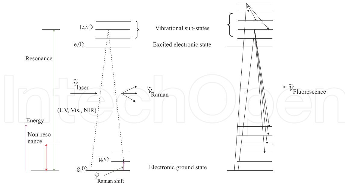
Fig. 3. Left: The Raman process is a coherent absorption-emission sequence. Right: Fluorescence is a real absorption followed by a spontaneous emission process, i.e. an incoherent absorption-emission sequence.
