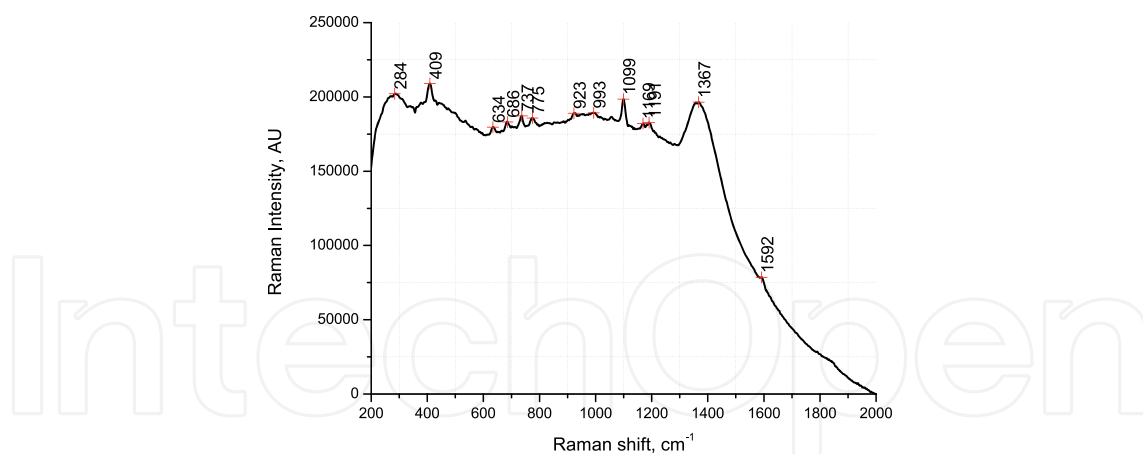
Fig. 14. A Raman spectrum of a pure dicofol powder, which was acquired with Inspector Raman. Notice the peak at 1099\text{ cm}^{-1} .
