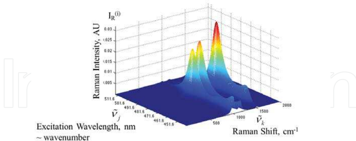
Fig. 4. RADIS, Raman spectra measured with a few different excitation wavelengths close to the electronic resonance of the chromophore.
