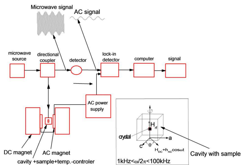
Fig. 1. Block diagram of the EPR spectrometer.
