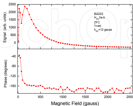
Fig. 5. AC induced microwave dissipation signal amplitude with the corresponding phase value of a Bi2223 single crystal, ZFC to 4K, as function of magnetic field aligned parallel to the a-b plane. The temperature behavior of the signals in Bi2223 is similar to that observed in Bi2212.
