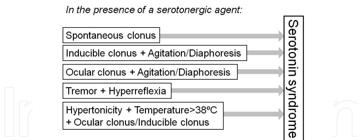
Fig. 3. Diagnostic criteria for SS proposed by Dunkley et al. (2003).
