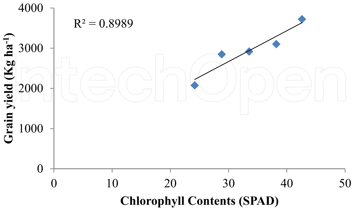
Fig. 5. Chlorophyll contents and grain yield of wheat genotypes under different silicon treatments
