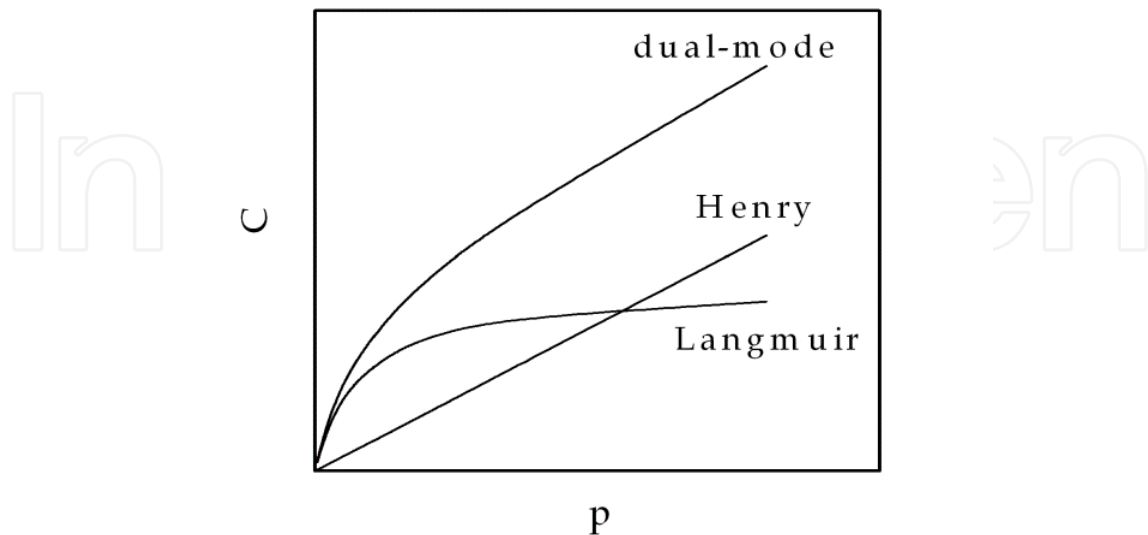
Fig. 1. Schematic representation of Henry, Langmuir, and dual-mode sorptions.
