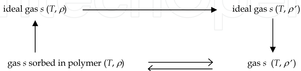
Scheme 1. Description of equilibrium between the gas s in the gaseous and polymeric phases.
