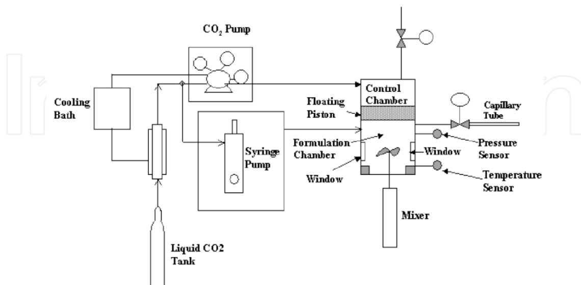
Fig. 5. Apparatus for preparation of OSN films by RESS technique (Reproduced from Ref. 51, Copyright 2006 Wiley-VCH Verlag GmbH & Co.)
