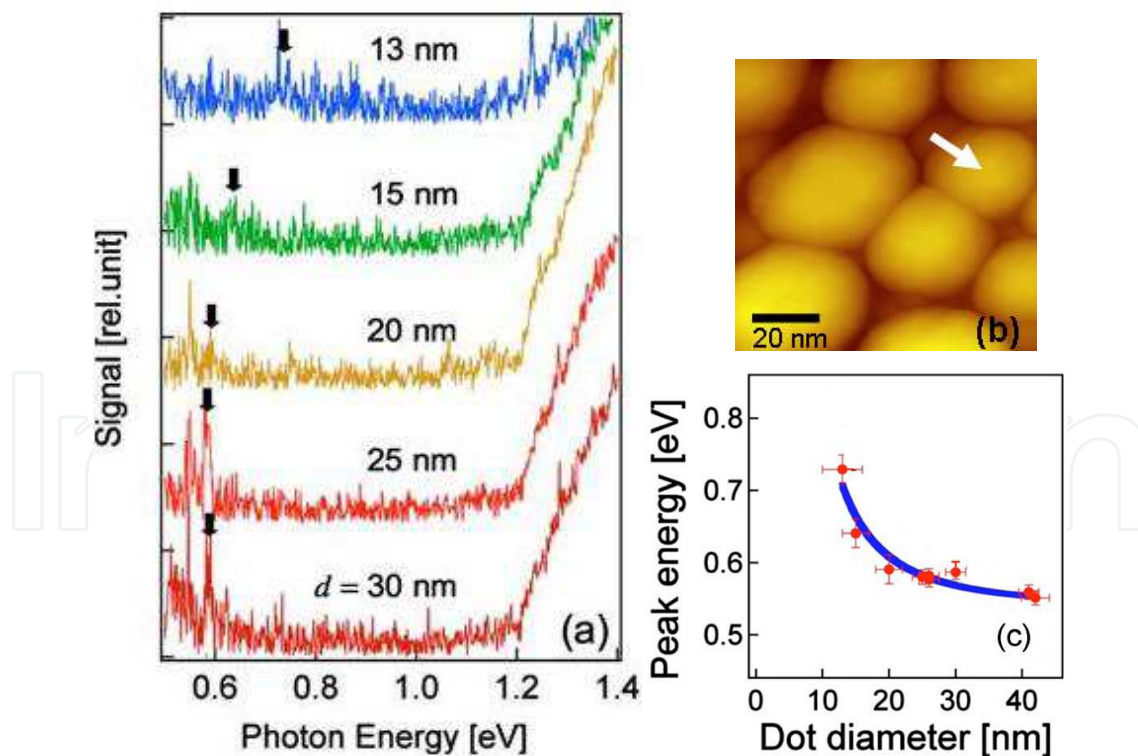
Fig. 3. (a) STM-PAS-FT spectra obtained from individual GeSn nanodots of various sizes. (b) Typical topographic STM image of \text{Ge}_{1-x}\text{Sn}_x nanodots. The white arrow indicates the position where the spectrum for d=30 nm was acquired. (c) Peak energy in (a) as a function of the lateral diameter of the nanodots. The solid curve is calculated from Eq. (1). [10]
