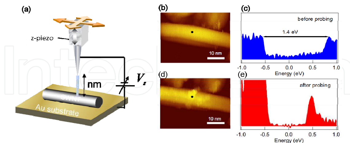
Fig. 14. (a) Schematic illustration of tunnel current injection. (b) STM image of an SWNT acquired with V_s=1.0 V and I_t=0.1 nA at 95 K. (c) dI/dV vs bias-voltage curve, obtained at the position marked in (b), exhibiting the features of a metallic SWNT characterized by a finite flat LDOS in the first van Hove gap. (d) STM image acquired after current injection at the marked position. (e) dI/dV vs bias-voltage curve, obtained at the position marked in (d), exhibiting a HOMO-LUMO gap of \sim 0.7 eV. [45]
