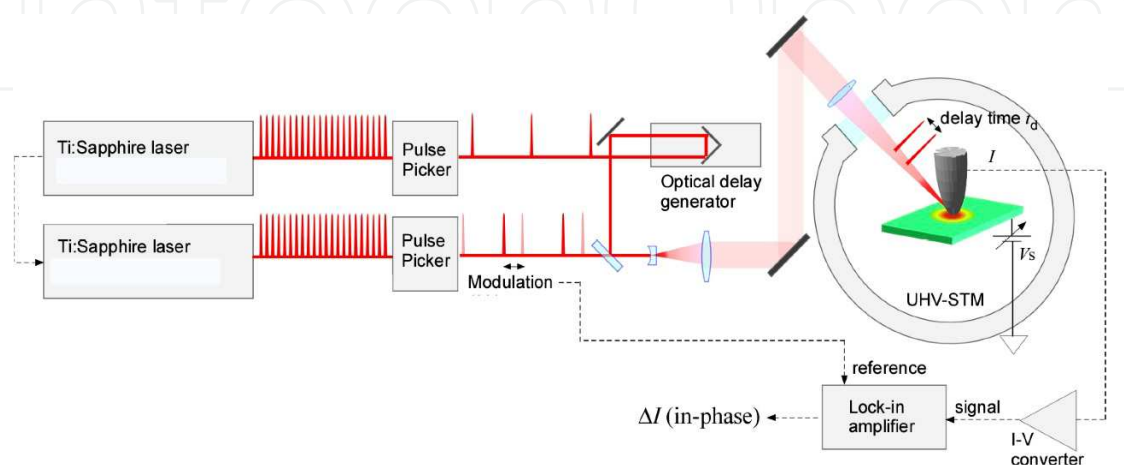
Fig. 9. Schematic illustration of SPPX-STM
