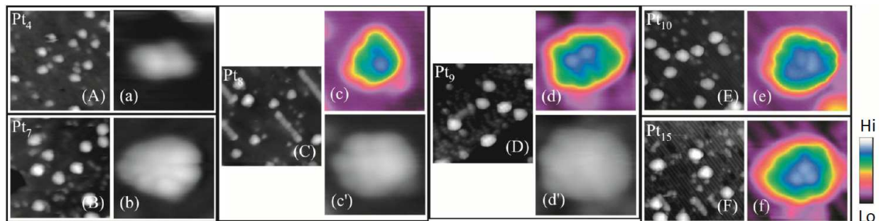
Fig. 15. STM images of \text{TiO}_2(110) surface after deposition of size-selected \text{Pt}_n^+ ( n = 4, 7-10, 15 ) cluster ions. Images with uppercase letters are 20 \times 20 \text{ nm}^2 views and those with lowercase letters are 3.5 \times 3.5 \text{ nm}^2 views of a cluster on the same surface. \text{TiO}_2 surface after the deposition of [(A), (a)] \text{Pt}_4^+ , [(B)(b)] \text{Pt}_7^+ , [(C)(c)(c')] \text{Pt}_8^+ , [(D)(d)(d')] \text{Pt}_9^+ , [(E)(e)] \text{Pt}_{10}^+ , [(F)(f)] \text{Pt}_{15}^+ [65].
