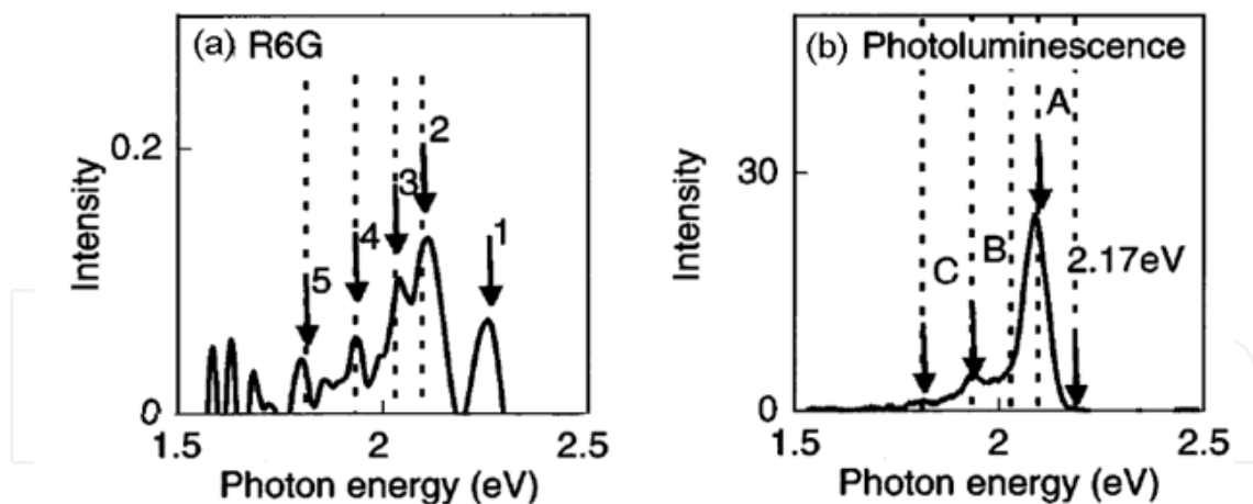
Fig. 8. (a) is the STM light emission spectrum of a single R6G molecule. (b) Photoluminescence (PL) spectrum of R6G on HOPG. The cutoff of the PL spectrum at 2.17 eV is due to the short-wavelength-cutoff filter inserted in the collection optics. [24]*
