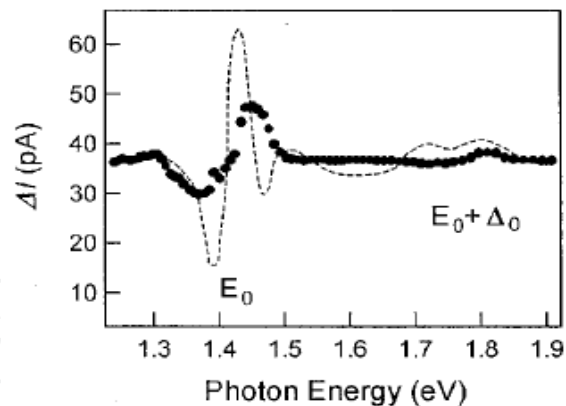
Fig. 5. STM-EFMS spectrum obtained for a perfect (110) cleaved surface of GaAs. The broken curve indicates the EFMS spectrum measured by the conventional electroreflectance method applied to a macroscopic GaAs sample. E_0 and E_0 + \Delta_0 denote the interband absorption edge of GaAs and to the spin split-off band absorption, respectively. [14]*
