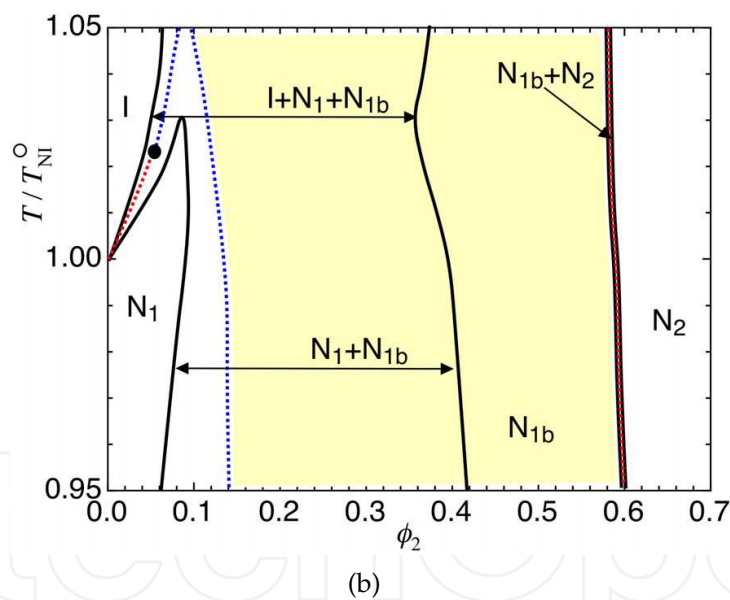
Fig. 11. Phase diagrams on the temperature ( \tau \equiv T/T_{NI}^0 )-volume fraction ( \phi_2 ) plane for c_{12} = -0.5 (a) and -0.8 (b). The black lines indicate the binodal. The red (blue) lines show a first (second)-order phase transition, where the order parameters discontinuously (continuously) change. The biaxial nematic phase N_{1b} , which includes an unstable biaxial phase, a metastable biaxial, and a stable biaxial phase, is indicated by the yellow area. The stable biaxial phase N_{1b} appears on (b).
