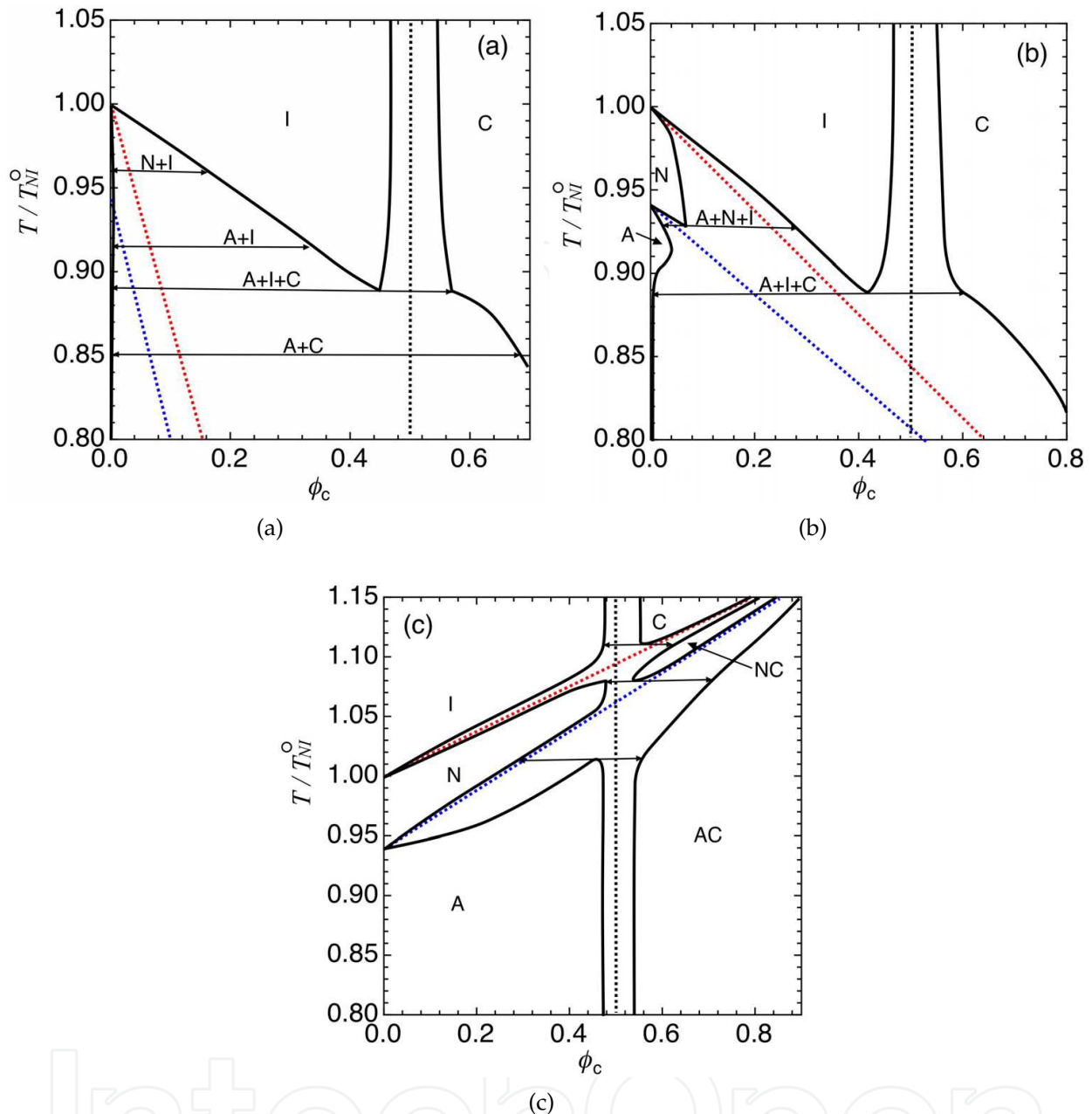
Fig. 4. Phase diagrams for \alpha_c = 0.1 , \alpha_n = 5 , \gamma = 0.87 . The value of \alpha_a is changed: (a) \alpha_a = 1 ; (b) \alpha_a = -2 ; (c) \alpha_a = -3.5 .
