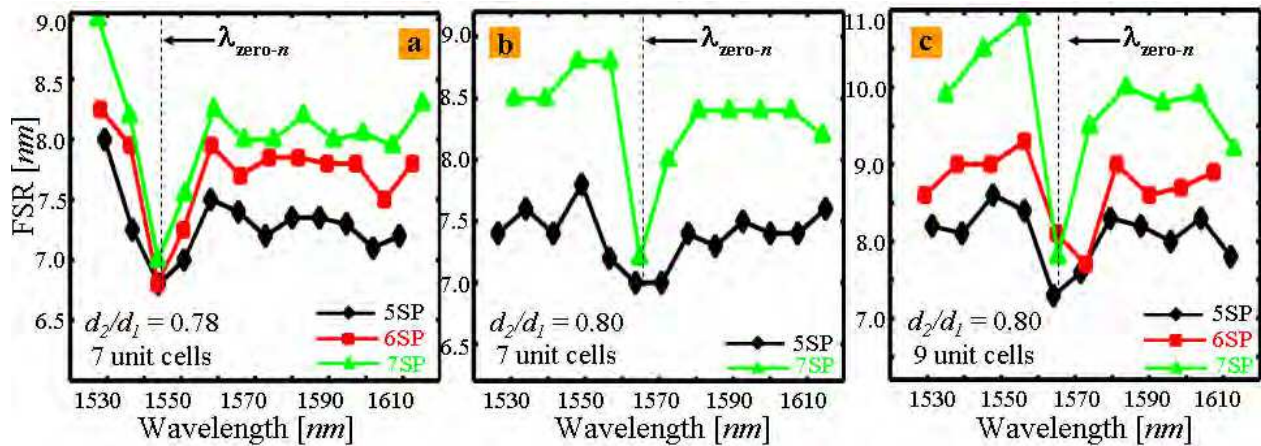
Fig. 12. Free spectral range wavelength dependence corresponding to superlattices in Figure 4. a-c, Free spectral range extracted from the data in Figure 4a-c. At the zero- n bandgap wavelength, the free spectral range converges to the same value, which proves the zero phase contribution from the added superperiods.
