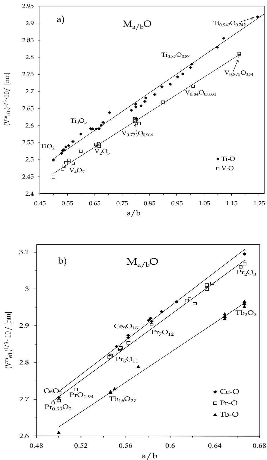
Fig. 8. The relation between the cube root of the molecular volume (V_{\text{eff}}^m)^{1/3} of oxide phases M_{a/b}O and the a/b ratio for the metal oxides: a) Ti and V, b) Ce, Pr and Tb.
