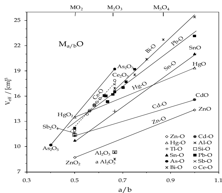
Fig. 4. The dependence of the effective molar volume ( V_{\text{eff}} ) of the oxides M_{a/b}\text{O} on the composition ( a/b ) for the group 11-15 metal oxides and Ce oxides.
