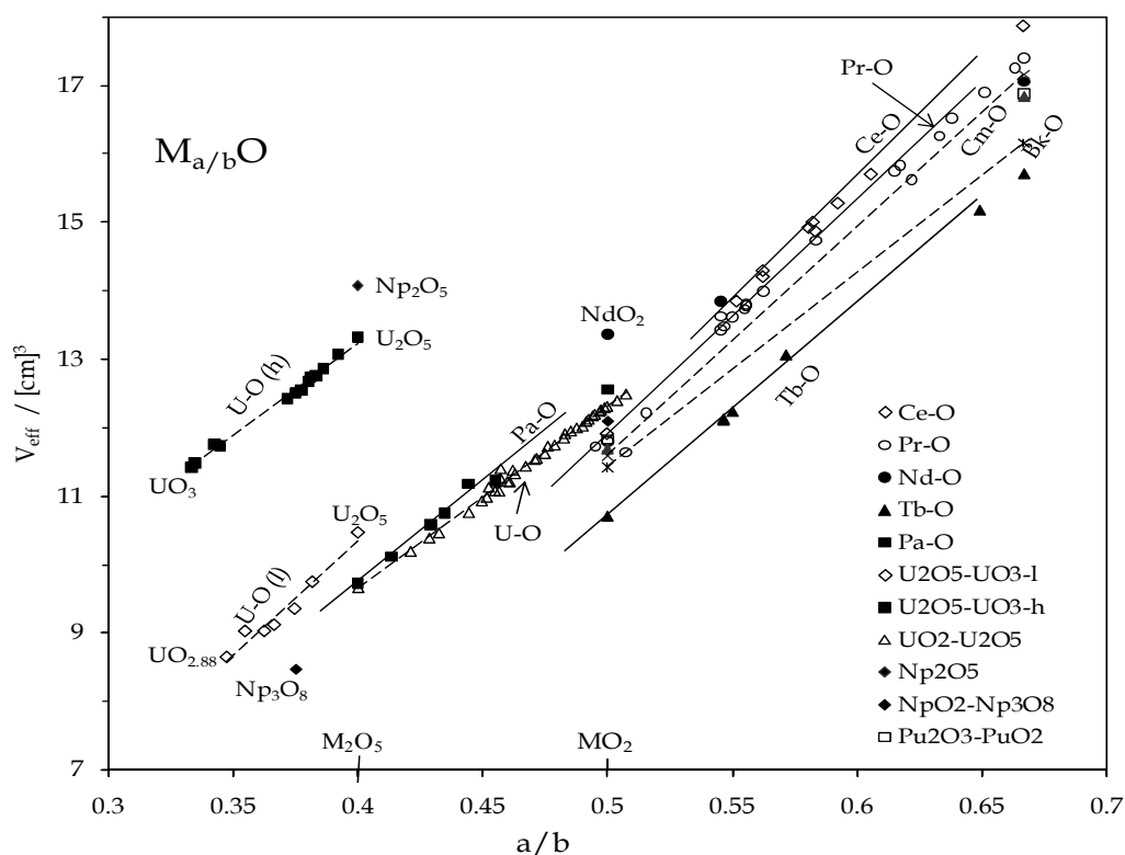
Fig. 2. The dependence of the effective molar volume ( V_{\text{eff}} ) of the oxides M_{a/b}O on the composition ( a/b ) for f -electron metal oxides, (—) - lanthanides, (- -) - actinides.
