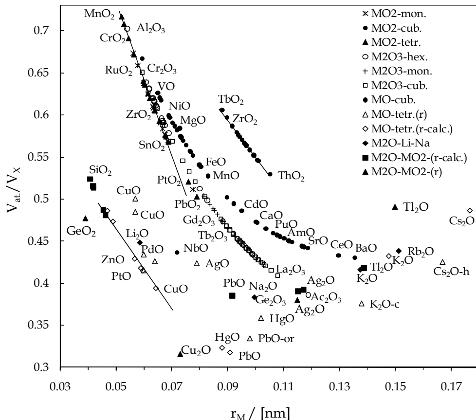
Fig. 10. The dependence of the packing density of a series of metal oxides with compact structures on the ionic radii calculated using relative ionic radii.
