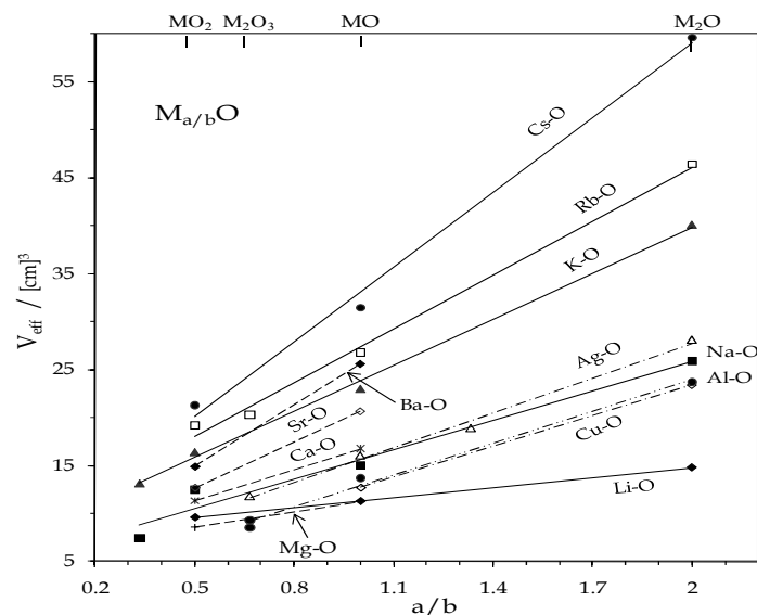
Fig. 3. The dependence of the effective molar volume ( V_{\text{eff}} ) of the oxides M_{a/b}\text{O} on the composition ( a/b ) for the alkali metal oxides, the oxides of Al, Ag, Cu and the alkaline earth metal oxides.
