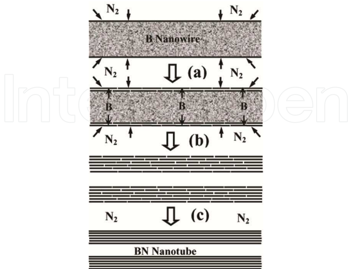
Fig. 11. Schematic diagram of the formation process of hollow BN nanotubes from solid boron nanowires.
