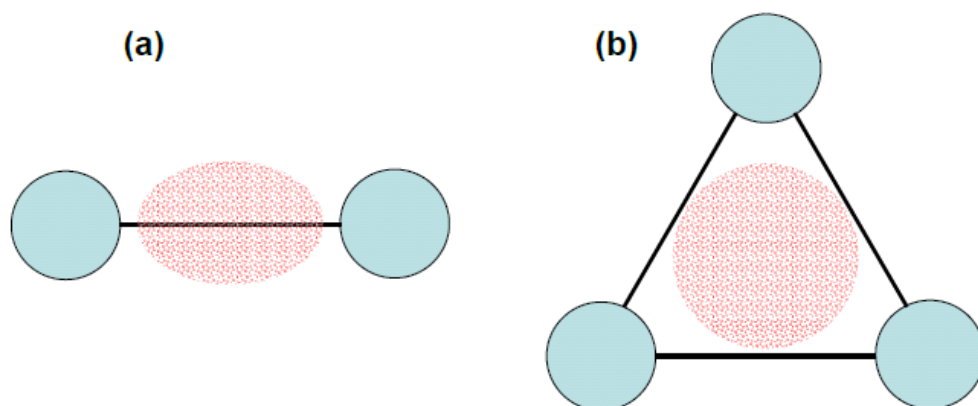
Fig. 1. Schematic of the electronic charge distributions (the dotted regions) of a two-center bond (a) and three-center bond (b).
