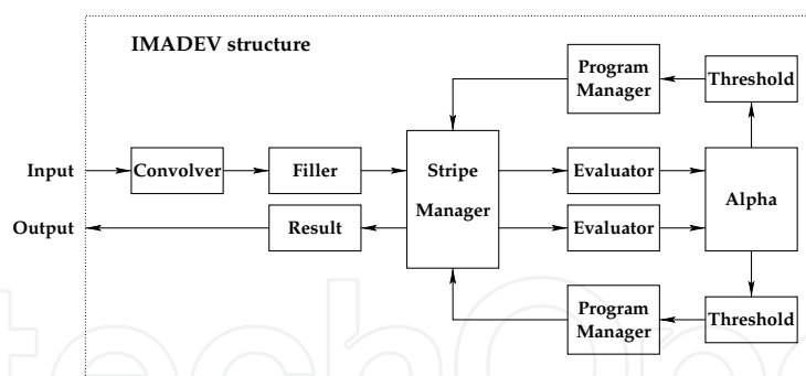
Fig. 6. Block structure of the object detector in programmable hardware (source Zemčík & Žádník (2007)).
