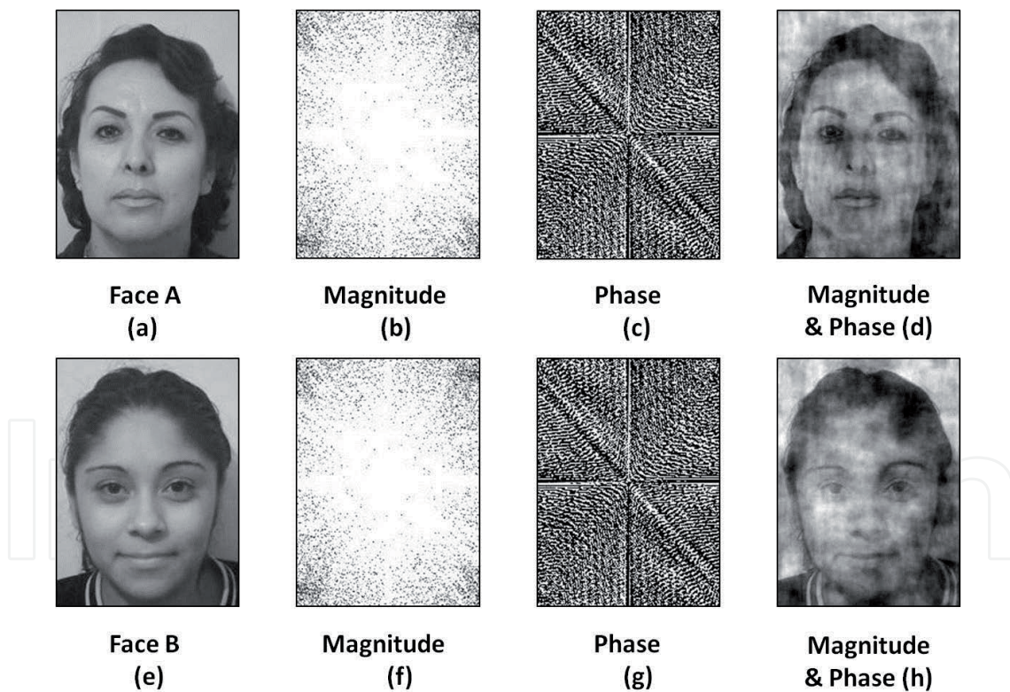
Fig. 6. Oppenheim Experiment
