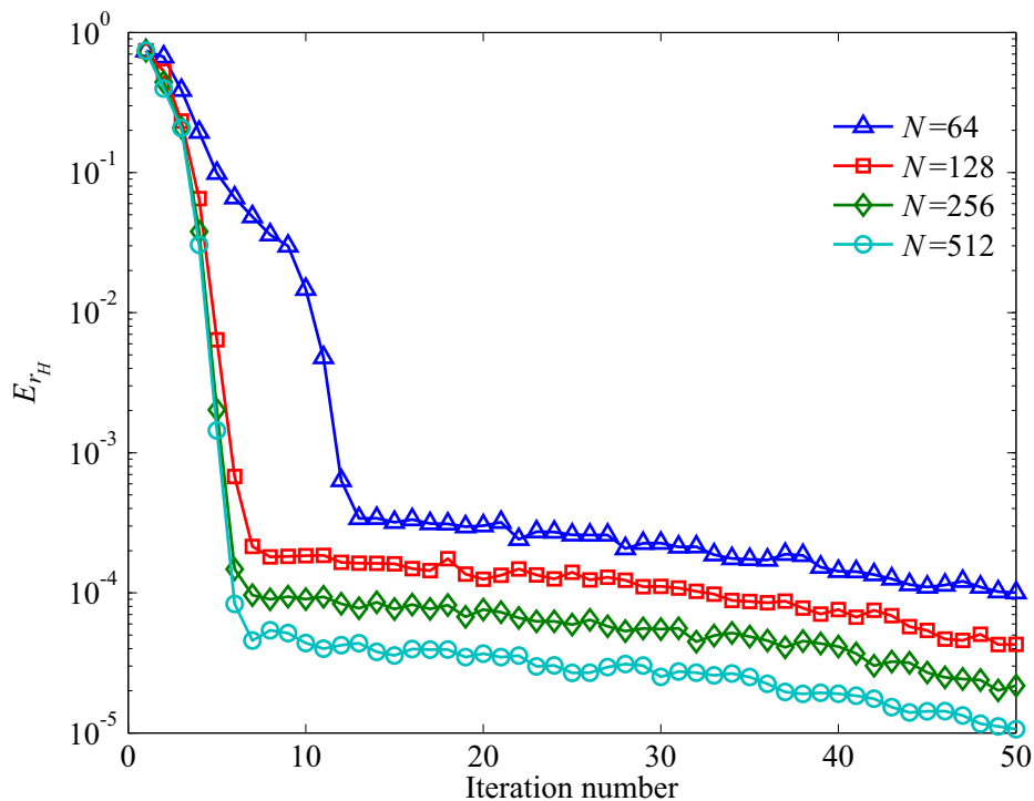
Fig. 9. Channel estimation error versus FFT size N
