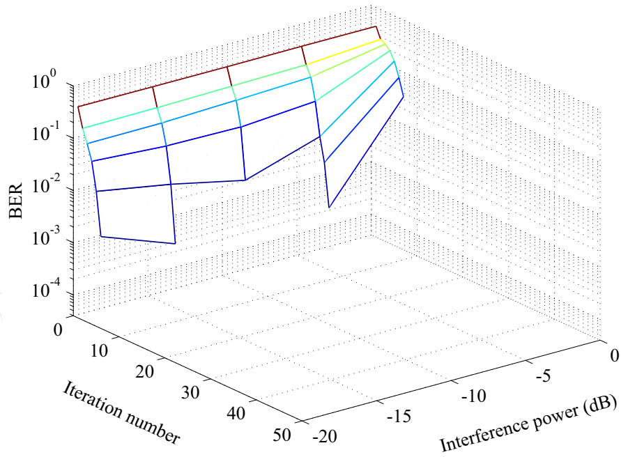
(b) Bit error rate
