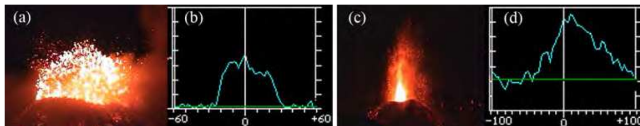
Fig. 7. Shapes of Doppler spectra associated with Strombolian activity. Outburst of a hemispherical lava bubble (a) and associated top-hat Doppler spectrum (b) at Etna's SE Crater (04/07/2001, 21:43'06). (c) Vertical lava jet at Laghetto (29/07/2001, 21:20'56) and the recorded triangular spectrum (d) (power in dBW vs. radial velocity in m/s).
