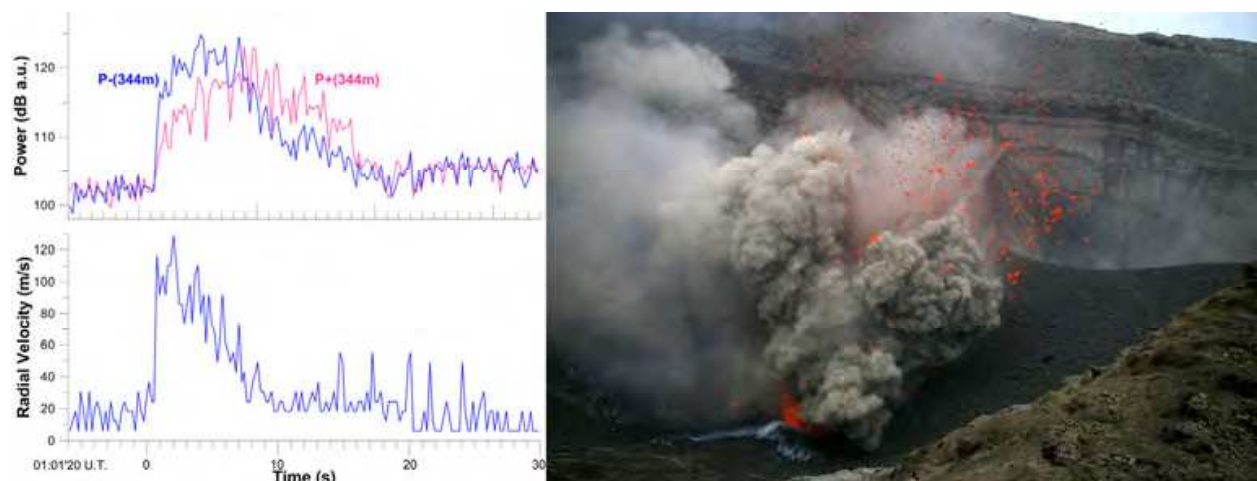
Fig. 10. ( left ): Time series of power ( top ) and maximum radial velocities ( bottom ) of a Strombolian outburst recorded by VOLDORAD aiming downward into Yasur's southern crater on 27/09/2008. Data are smoothed with 3 incoherent integrations (0.21 s).
