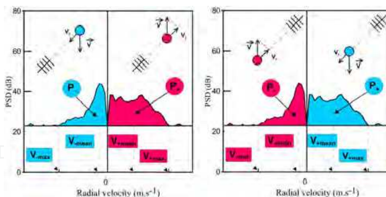
Fig. 6. Volcanic particle contributions to Doppler spectra in different sounding conditions. (a) When the antenna points upward (e.g. at summit craters from the flanks), ascending volcanic particles in red induce echoes with an along-beam velocity component away from the radar (positive radial velocity range, right part of spectrum), whereas falling particles in blue induce radial velocities toward the radar (negative radial velocity range, left part of spectrum). (b) The contributions are reversed when the antenna beam points downward (e.g. down towards a crater from the rim).
