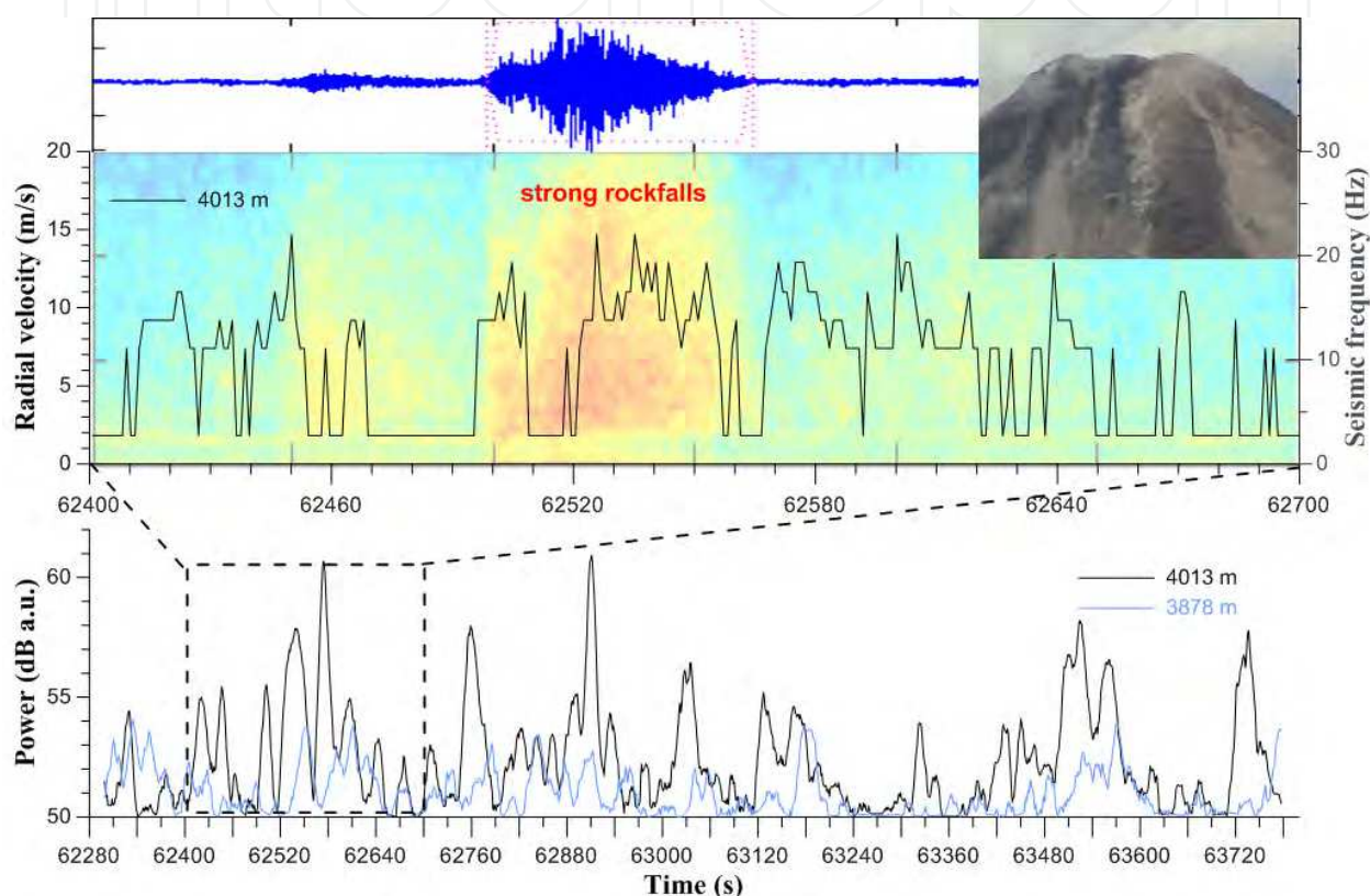
Fig. 17. Radar and seismic signals associated with rock falls at Arenal (02/02/2009). Bottom : 25 minute record of power from two range gates hitting the volcano upper slopes, where rock falls are detected by VOLDORAD; middle : maximum radial velocity (component towards radar) superimposed on a color spectrogram showing the seismic frequency content associated with rock fall events; top : seismic trace of a large rock fall and view of Arenal's summit from north showing lava flows and rock falls producing dust (seismic data courtesy of M. Mora; photo © F. Donnadieu, 14/05/2006).
