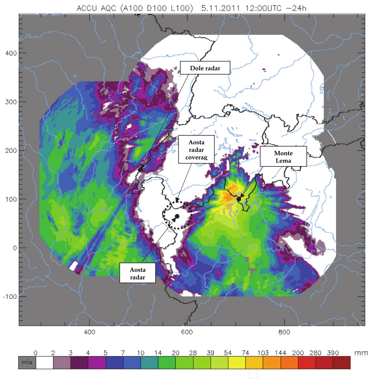
Fig. 3a. 24-hour cumulative rainfall amounts in the western Alps as seen by the Swiss weather radar network (from 12 UTC of November 4 to 12 UTC of November 5, 2011). North and East axes map units are in km.
