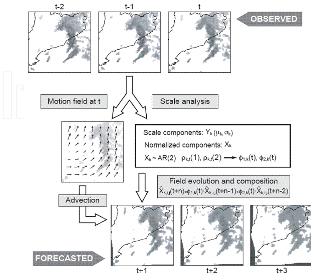
Fig. 2. The generation of an extrapolation nowcast using the Spectral-Prognosis (Seed, 2003) multi-scale decomposition (cascade) framework (after Berenguer et al., 2005). The motion of the precipitation field is derived from radar inferred analyses of precipitation rate valid at t and t-1 (typically a 10 or 15 minute time step). The temporal evolution of the extrapolated field is modelled on the hierarchy of scales produced by the cascade decomposition, using a hierarchy of second order auto-regressive (AR-2) models – one for each scale – and the analyses of precipitation rate valid at t , t-1 and t-2 .
