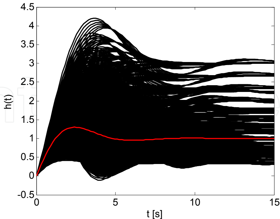
Fig. 2. Step responses of 2402 systems from interval family (1)
