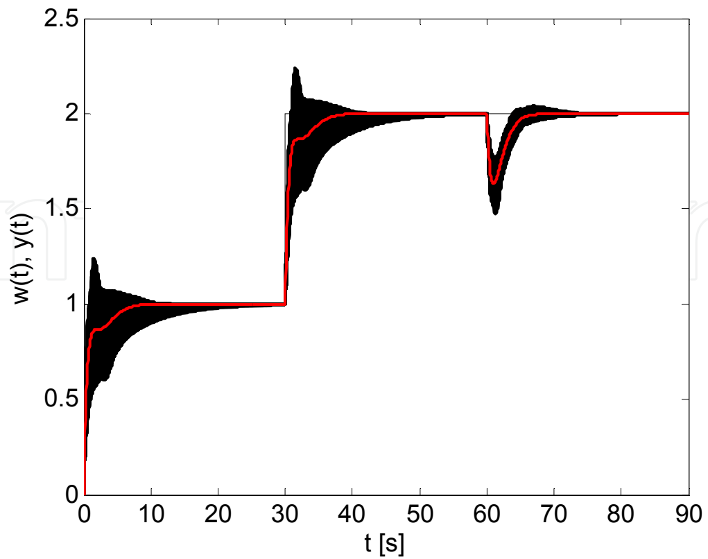
Fig. 9. Control of RSS of interval family (1) and nominal system by controller (2)
