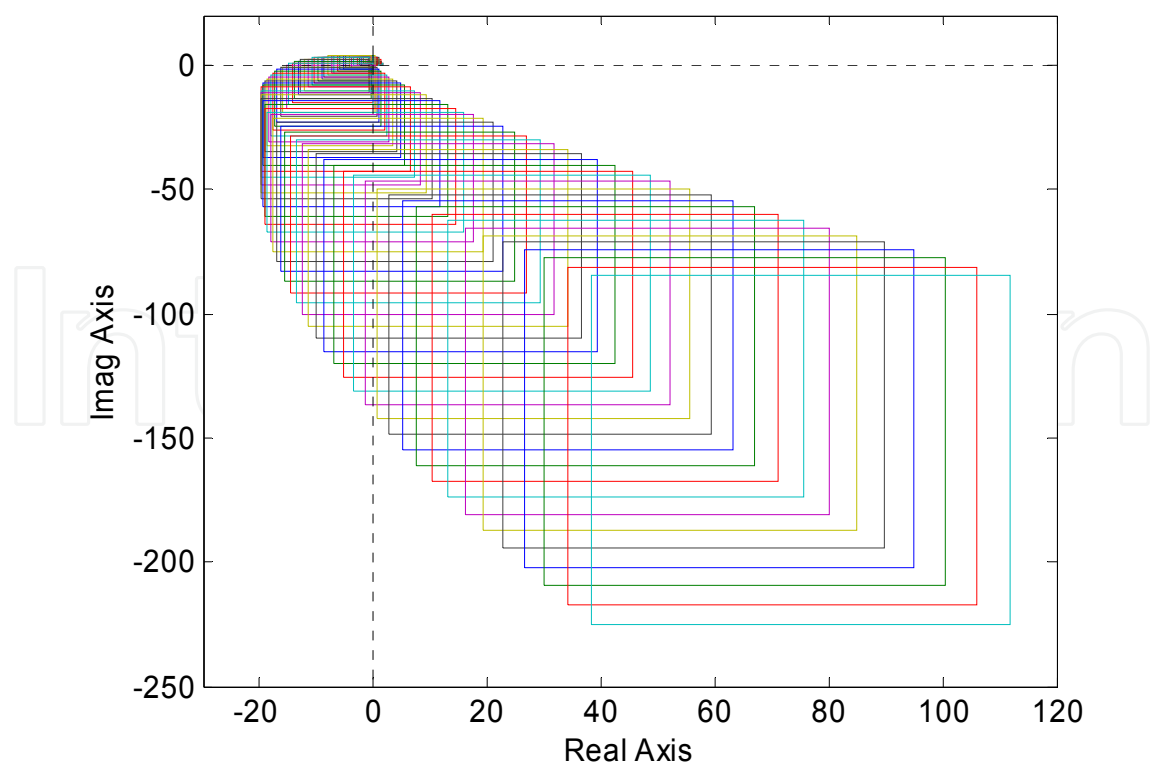
Fig. 4. The Kharitonov rectangles of overbounding interval polynomial - full view
