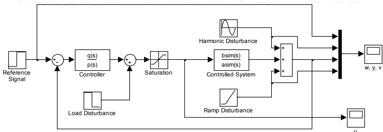
Fig. 8. Simulink scheme of 1DOF control system
