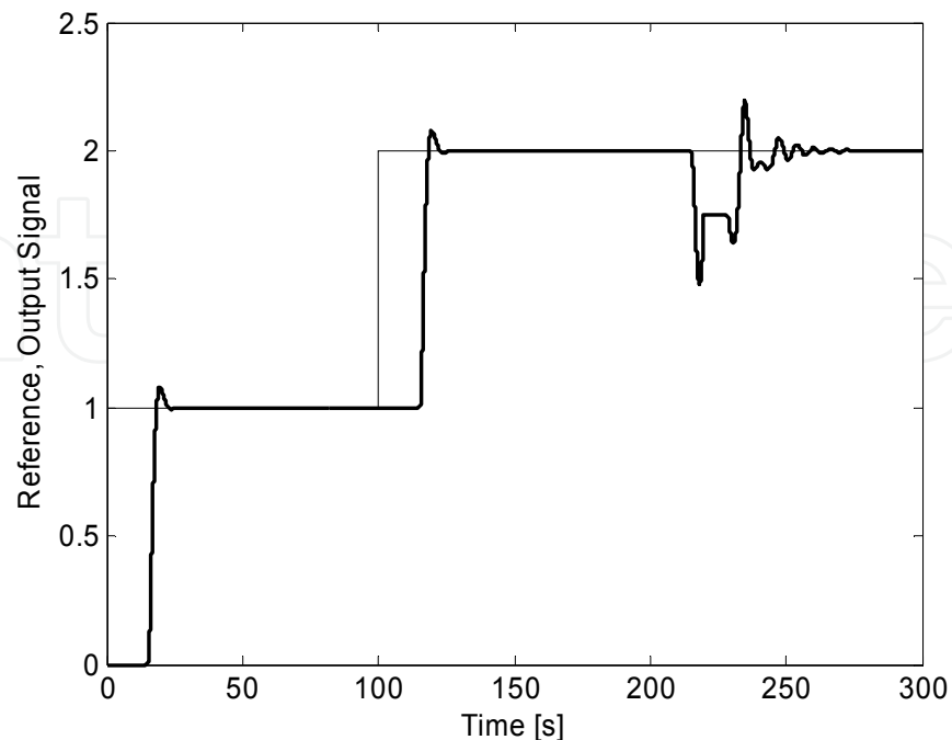
Fig. 17. Control results for system (7)
