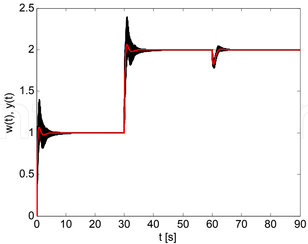
Fig. 10. Control of RSS of interval family (1) and nominal system by controller (7) - 1DOF
