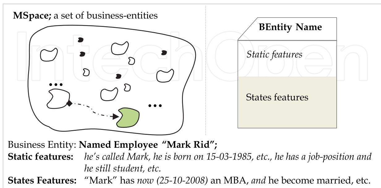
Fig. 1. MSpace basis
