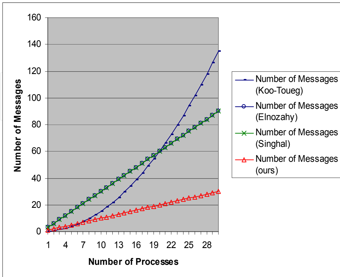
Fig. 5. Number of messages vs. number of processes for four different approaches when C_{\text{broad}} = n * C_{\text{air}}
